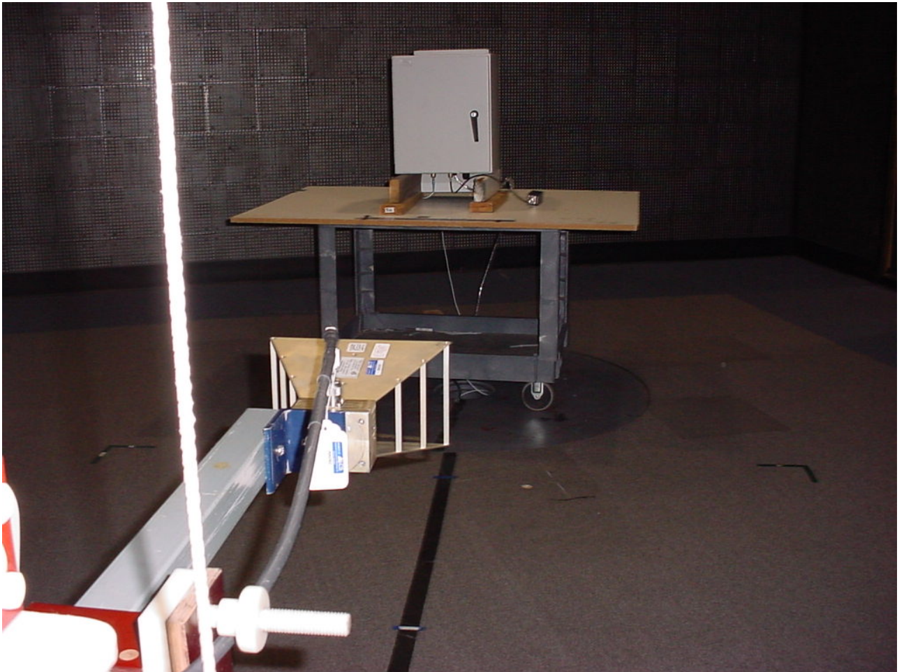
Figure 1: Test Setup - Radiated Emissions - Intentional
