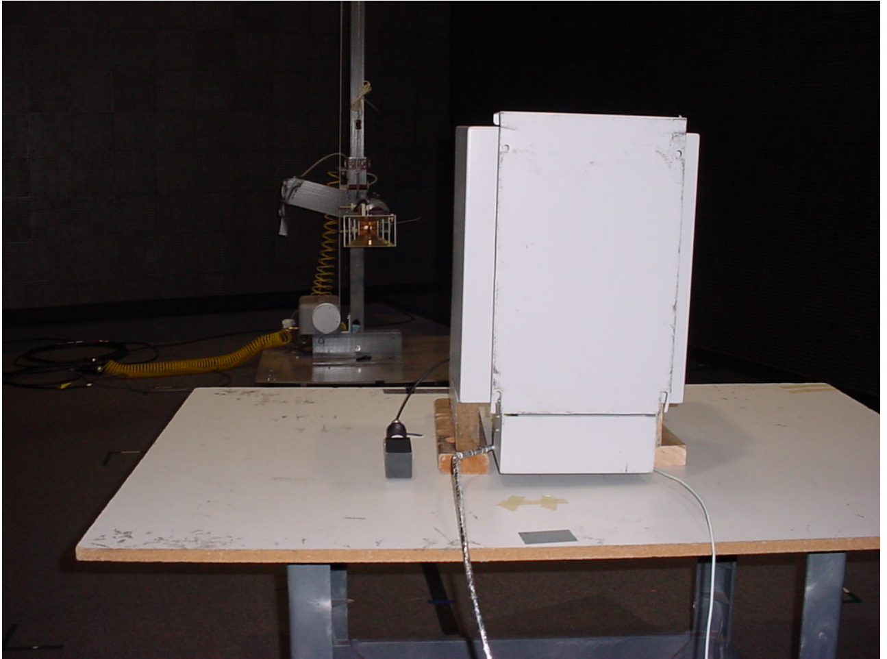
Figure 2: Test Setup - Radiated Emissions - Intentional
