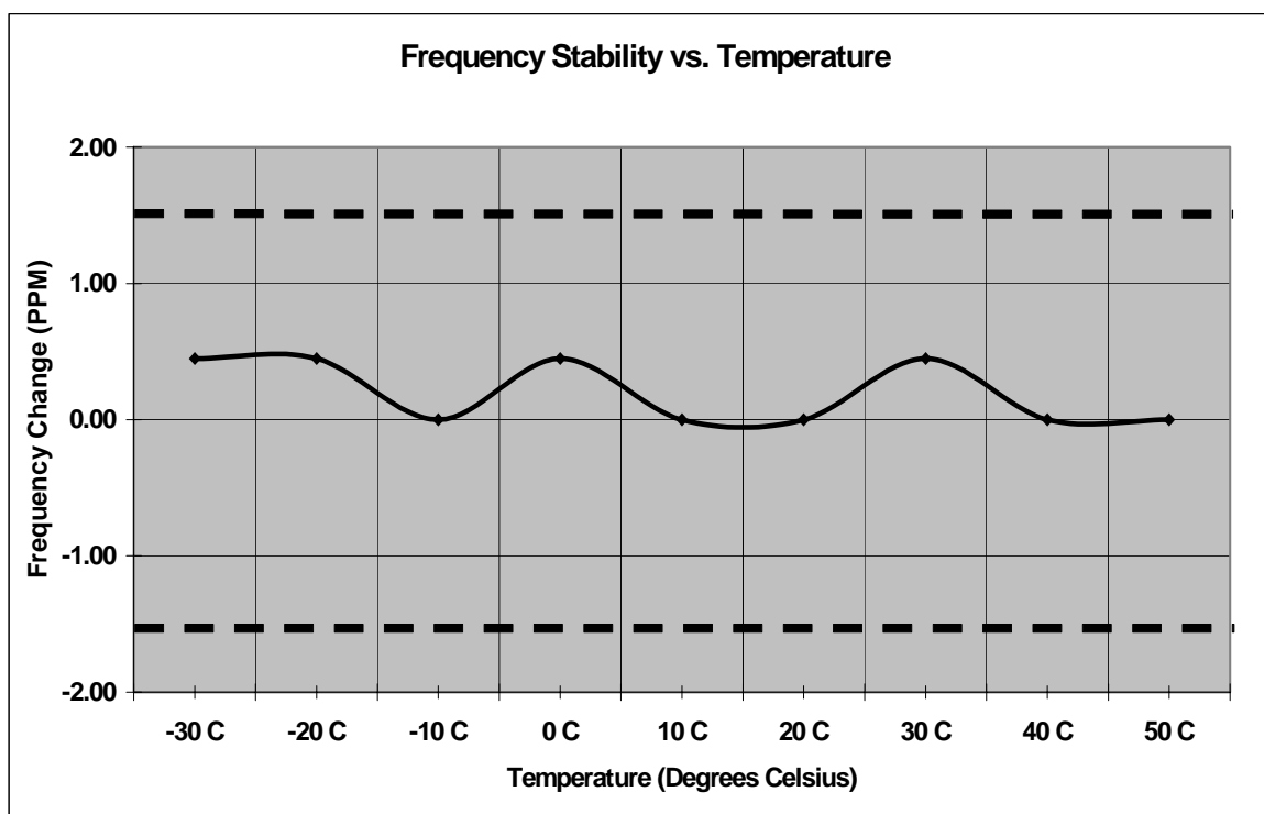
Figure 7.8-3: Frequency Stability Downlink – High Channel
