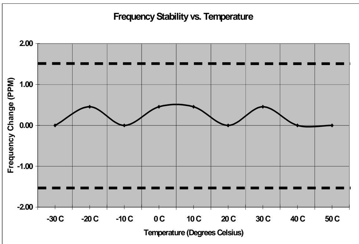
Figure 7.8-2: Frequency Stability Downlink – Middle Channel
