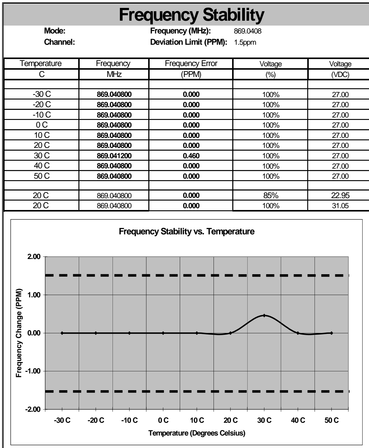
Figure 7.8-1: Frequency Stability Downlink – Low Channel
