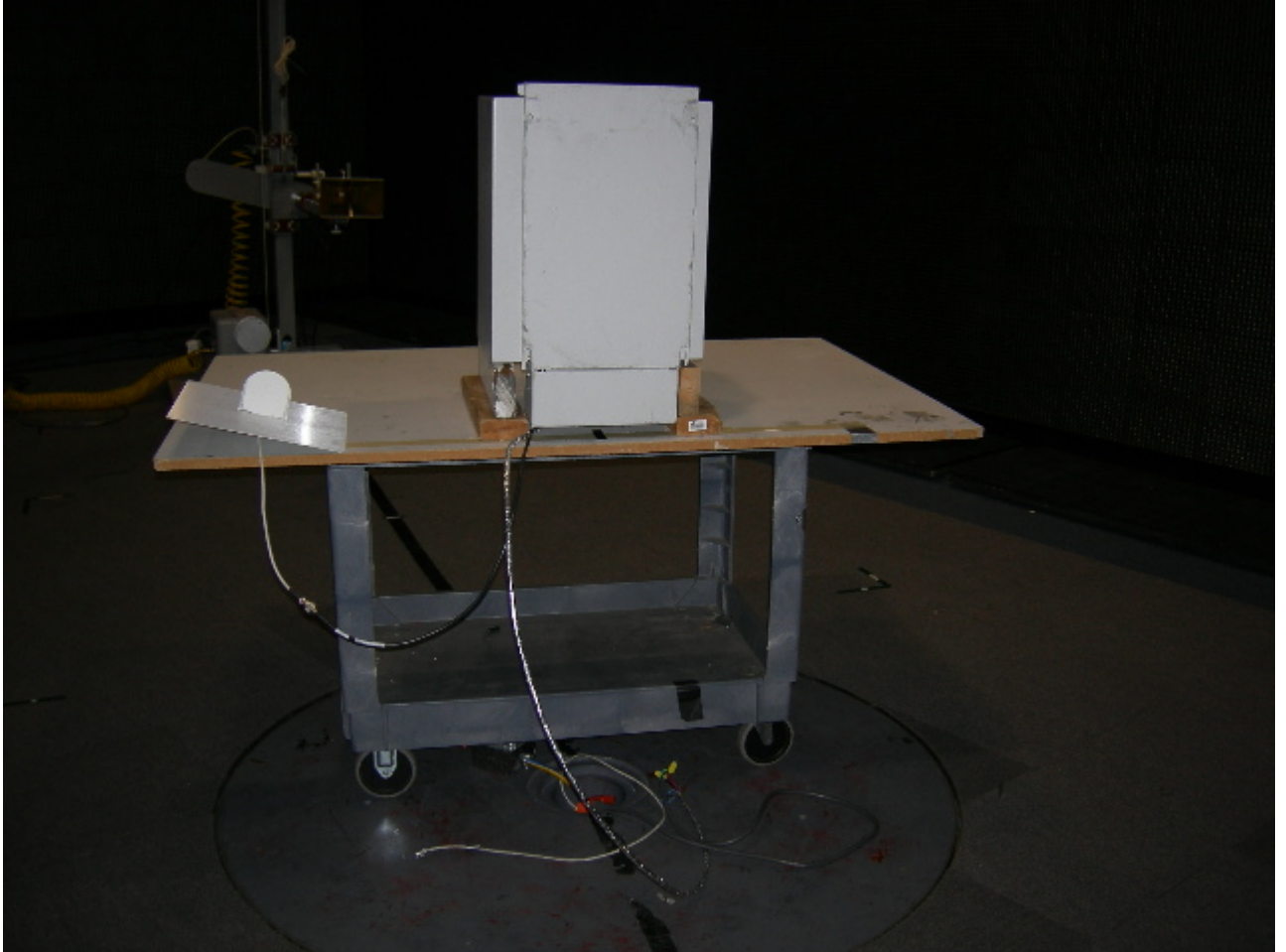
Figure 4: Test Setup - Radiated Emissions - Unintentional
