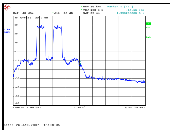
Figure 15: Spurious Emissions - Downlink CDMA High Channel – Inter-modulation In Band
