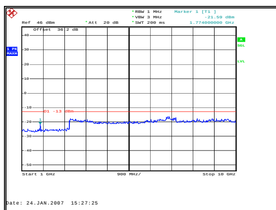
Figure 22: Spurious Emissions - Downlink TDMA Mid Channel – 1 to 10 GHz
