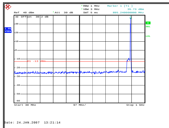
Figure 36: Spurious Emissions - Downlink GSM High Channel – 30 MHz to 1 GHz
