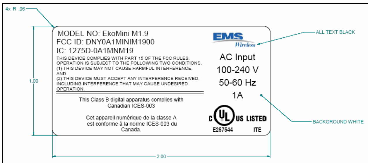
Figure 2: Label Sample
