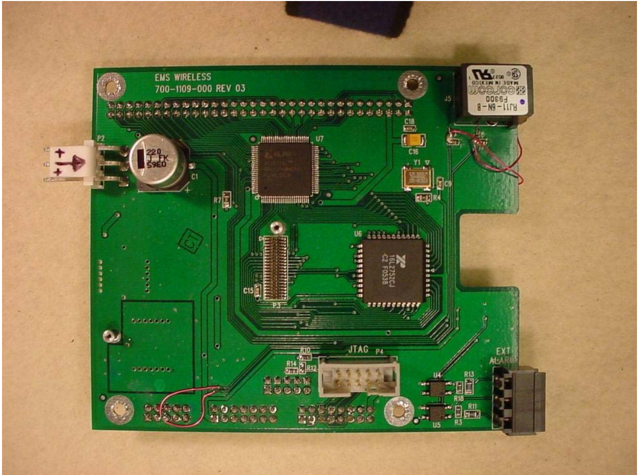
Figure 5: Internal – Modem RF Deck w/o modem Front
