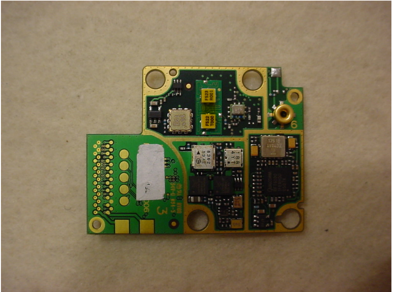
Figure 9: Internal – Modem w/o Shield Front
