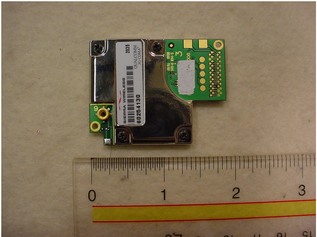
Figure 7: Internal – Modem w/ Shield Front
