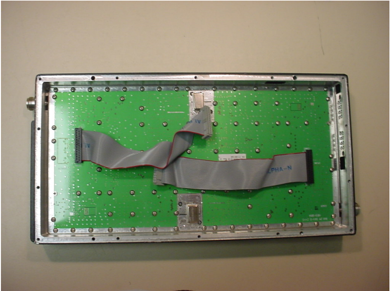
Figure 1: Internal – Booster RF Deck Front
