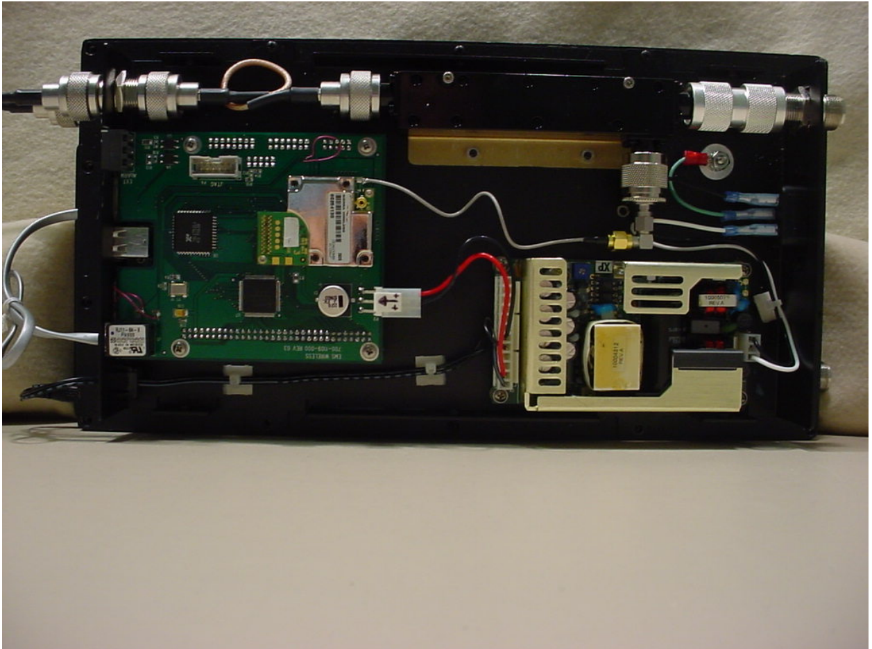
Figure 3: Internal – Modem Section Assembled
