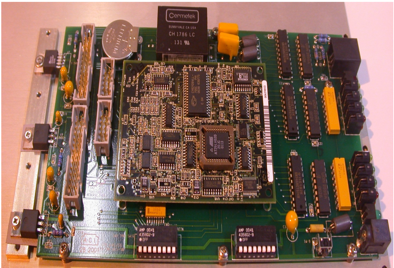
Figure 3: Internal – Microcontroller Front - Assembled
