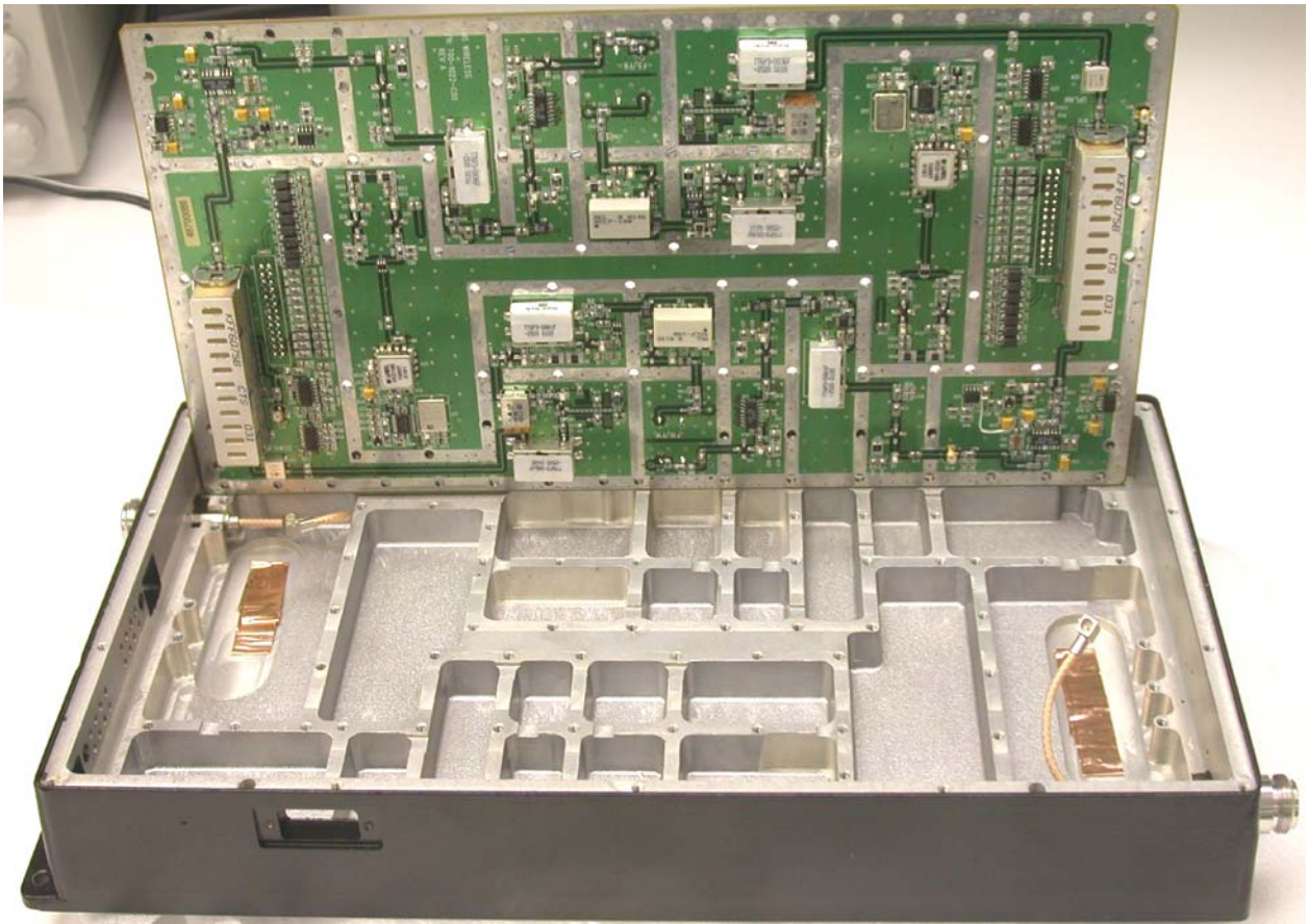
Figure 2: Internal – RF Deck Back
