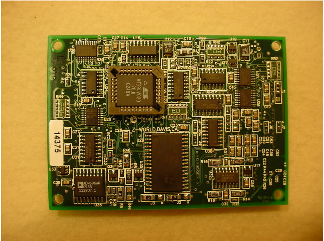
Figure 6: Internal – Microcontroller Front – Upper Board
