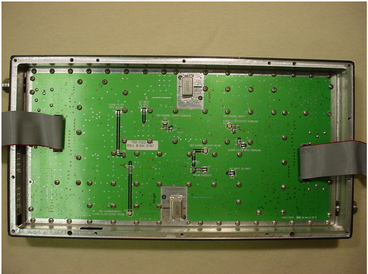
Figure 1: Internal – RF Deck Front
