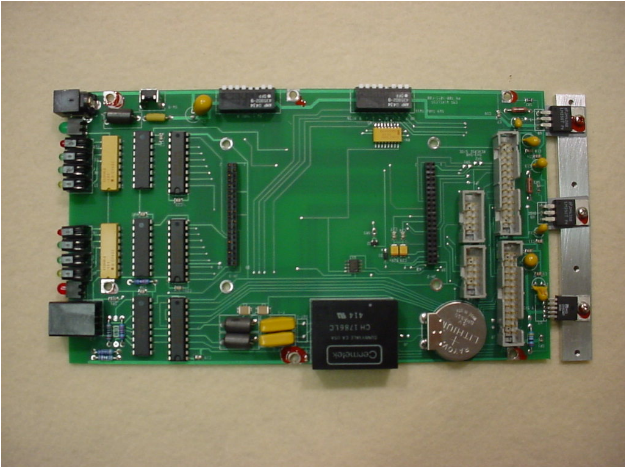
Figure 4: Internal – Microcontroller Front – Lower Board
