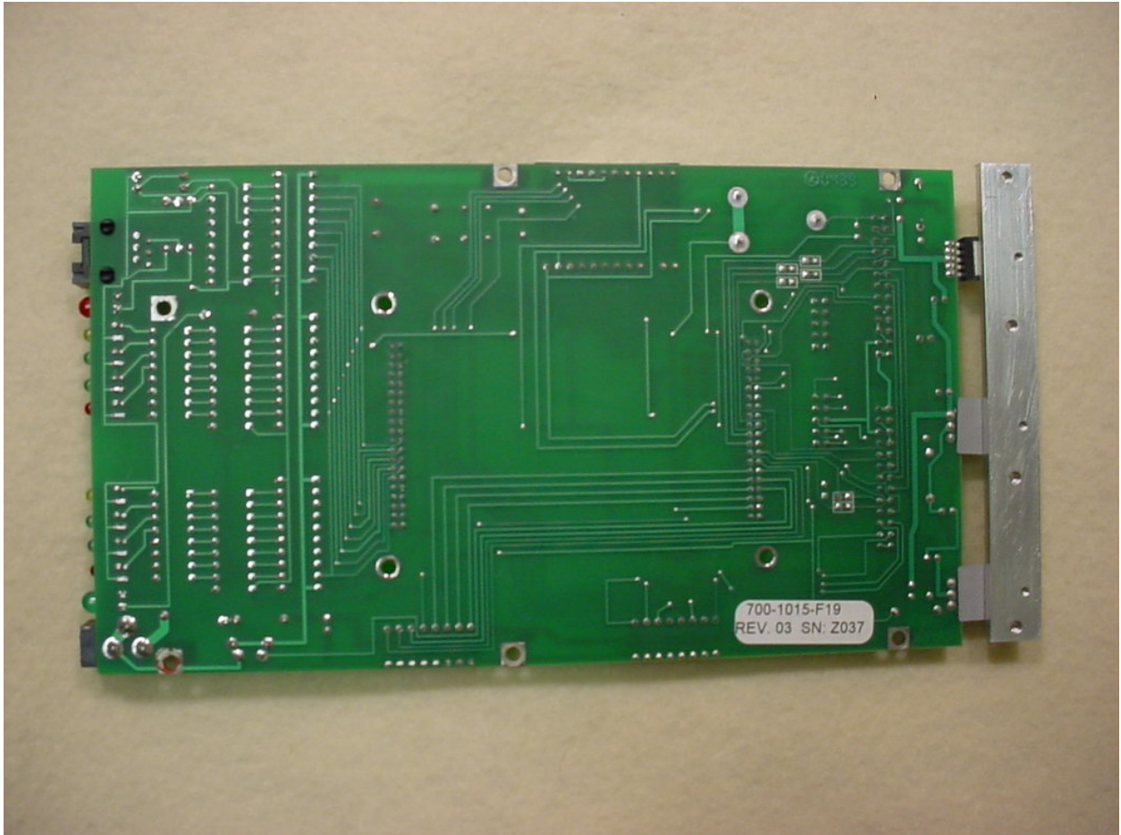
Figure 5: Internal – Microcontroller Back – Lower Board
