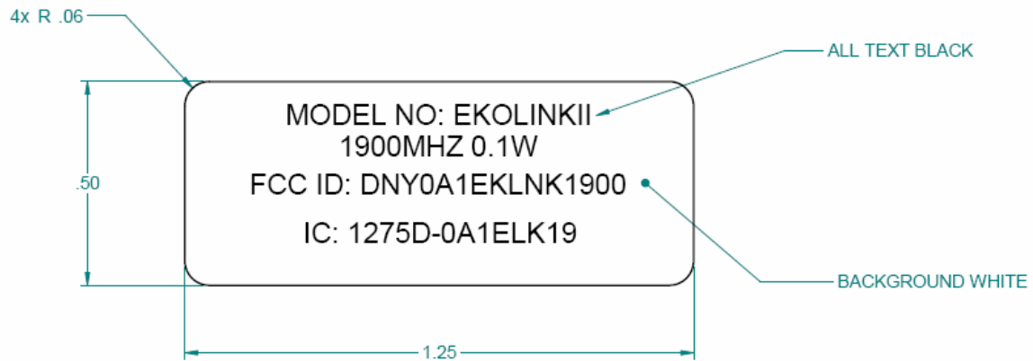
Figure1: FCC ID Label
