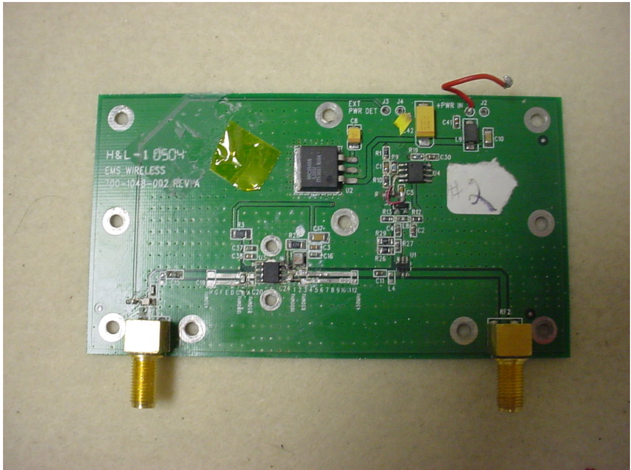
Figure 2: Internal – Amplifier Top View
