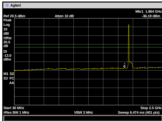
Figure 5: Spurious Emissions - CDMA Low Channel – 30 MHz to 2.5 GHz
