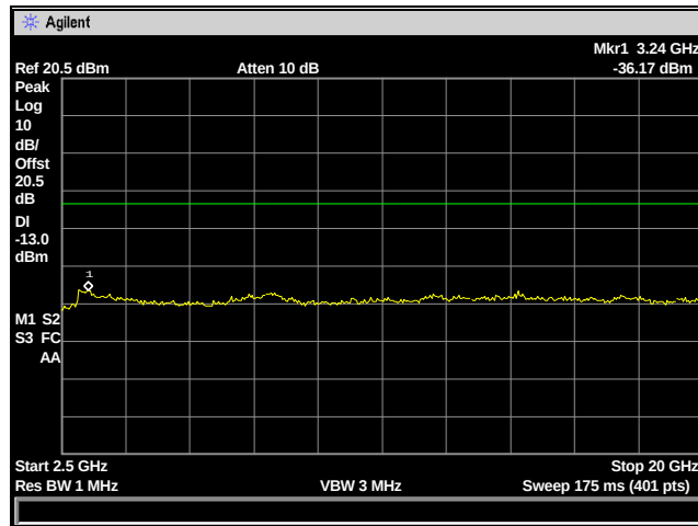
Figure 22: Spurious Emissions - GSM Low Channel – 2.5 to 20 GHz
