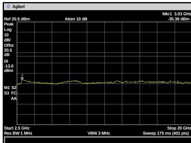
Figure 24: Spurious Emissions - GSM Mid Channel – 2.5 to 20 GHz
