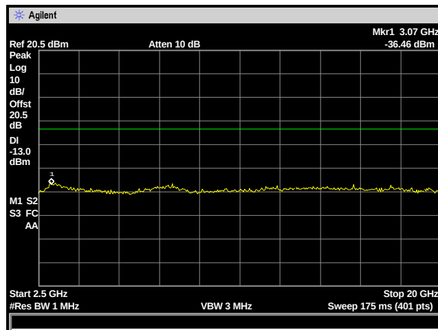
Figure 20: Spurious Emissions – CW Low Channel – 2.5 to 20 GHz
