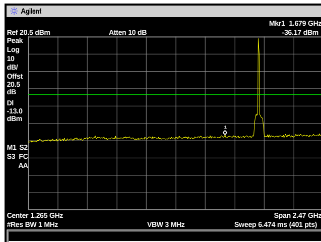
Figure 14: Spurious Emissions - TDMA Mid Channel – 30 MHz to 2.5 GHz
