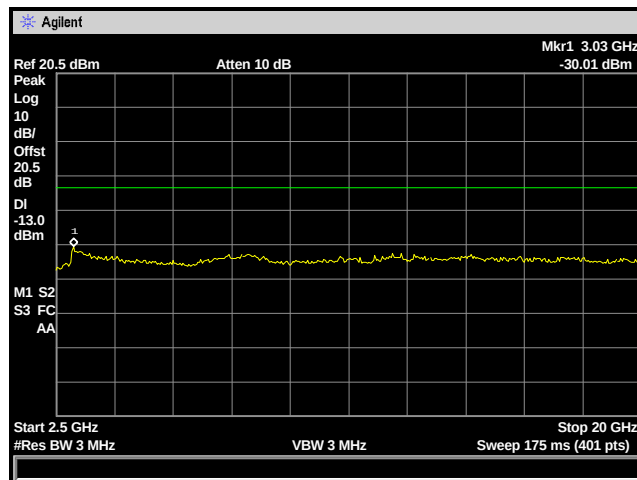
Figure 17: Spurious Emissions - TDMA High Channel – 2.5 to 20 GHz
