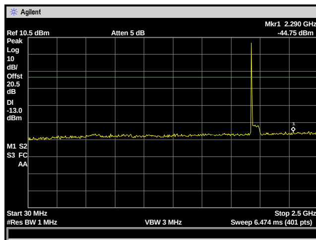
Figure 12: Spurious Emissions - TDMA Low Channel – 30 MHz to 2.5 GHz
