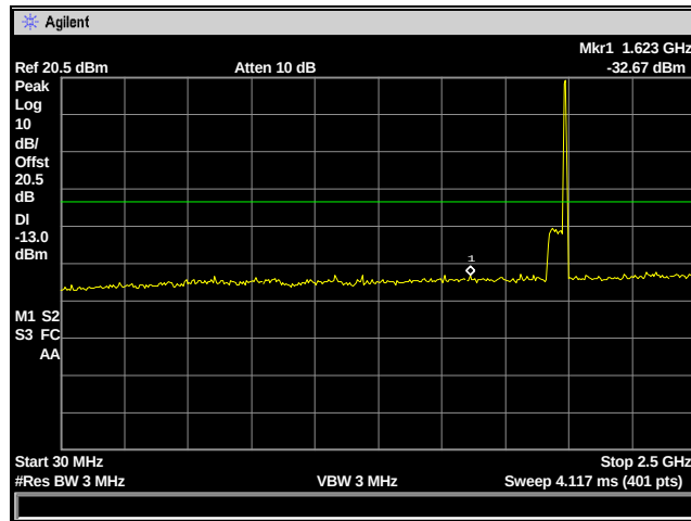
Figure 16: Spurious Emissions - TDMA High Channel – 30 MHz to 2.5 GHz
