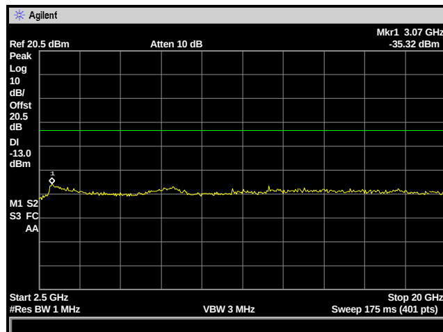
Figure 15: Spurious Emissions - TDMA Mid Channel – 2.5 to 20 GHz
