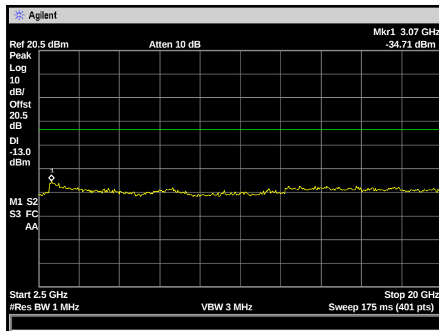
Figure 8: Spurious Emissions - CDMA Mid Channel – 2.5 to 20 GHz
