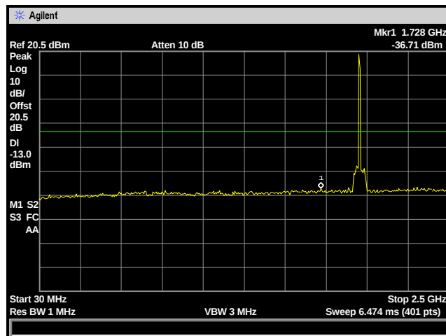
Figure 23: Spurious Emissions - GSM Mid Channel – 30 MHz to 2.5 GHz
