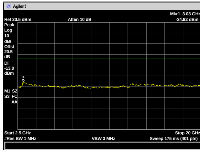
Figure 10: Spurious Emissions - CDMA High Channel – 2.5 to 20 GHz
