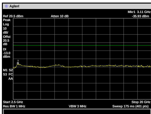
Figure 26: Spurious Emissions - GSM High Channel – 2.5 to 20 GHz
