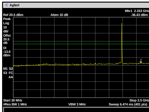
Figure 9: Spurious Emissions - CDMA High Channel – 30 MHz to 2.5 GHz
