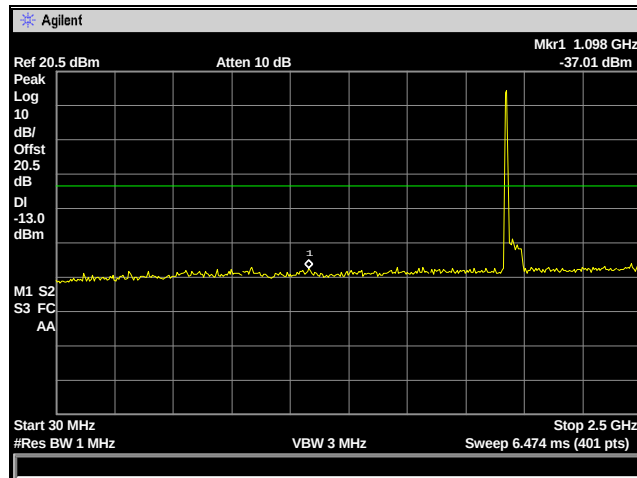
Figure 19: Spurious Emissions – CW Low Channel – 30 MHz to 2.5 GHz
