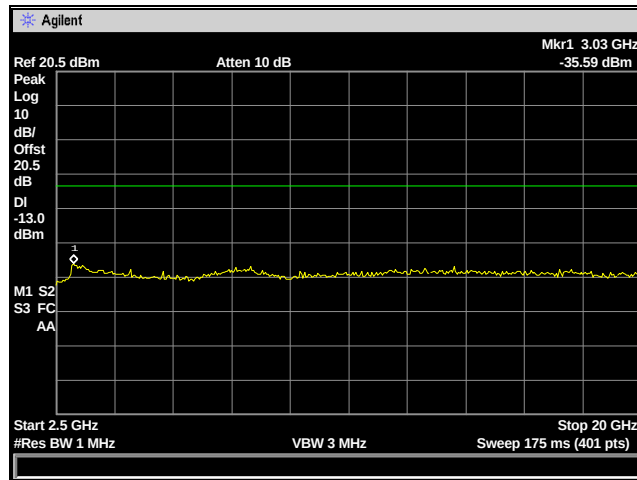
Figure 13: Spurious Emissions - TDMA Low Channel – 2.5 to 20 GHz
