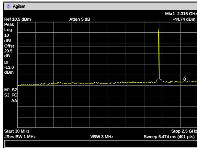
Figure 7: Spurious Emissions - CDMA Mid Channel – 30 MHz to 2.5 GHz
