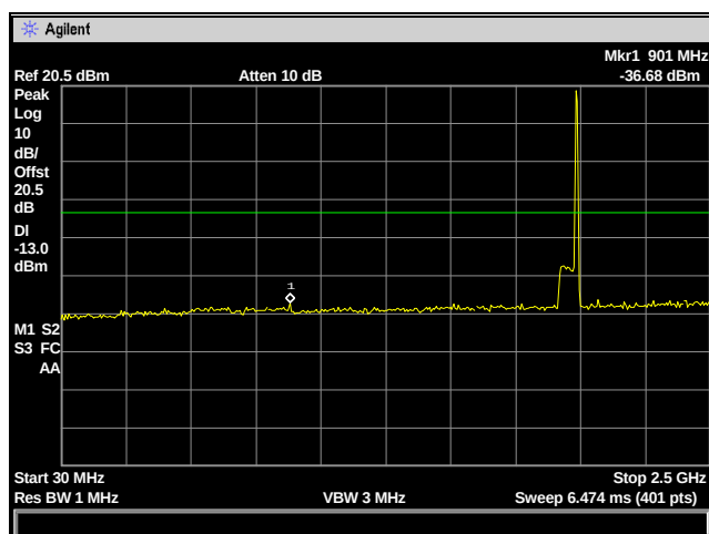
Figure 25: Spurious Emissions - GSM High Channel – 30 MHz to 2.5 GHz
