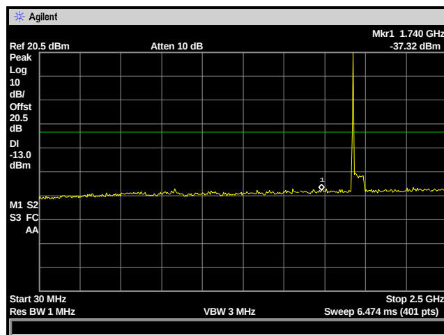
Figure 21: Spurious Emissions - GSM Low Channel – 30 MHz to 2.5 GHz
