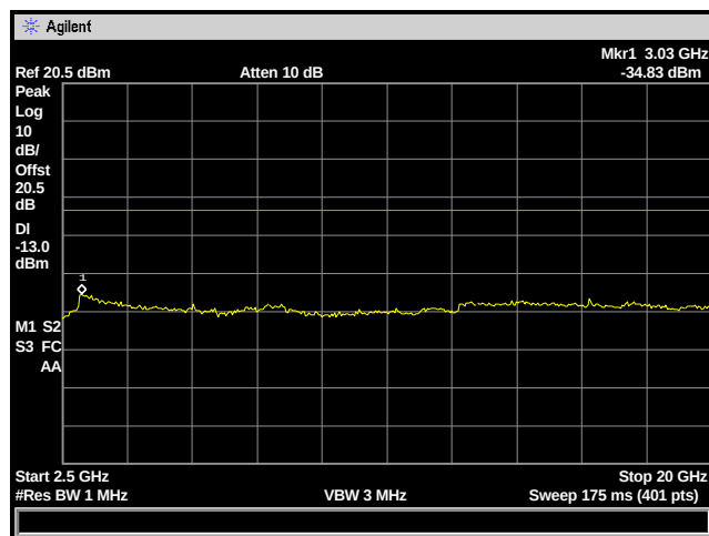
Figure 6: Spurious Emissions - CDMA Low Channel – 2.5 to 20 GHz
