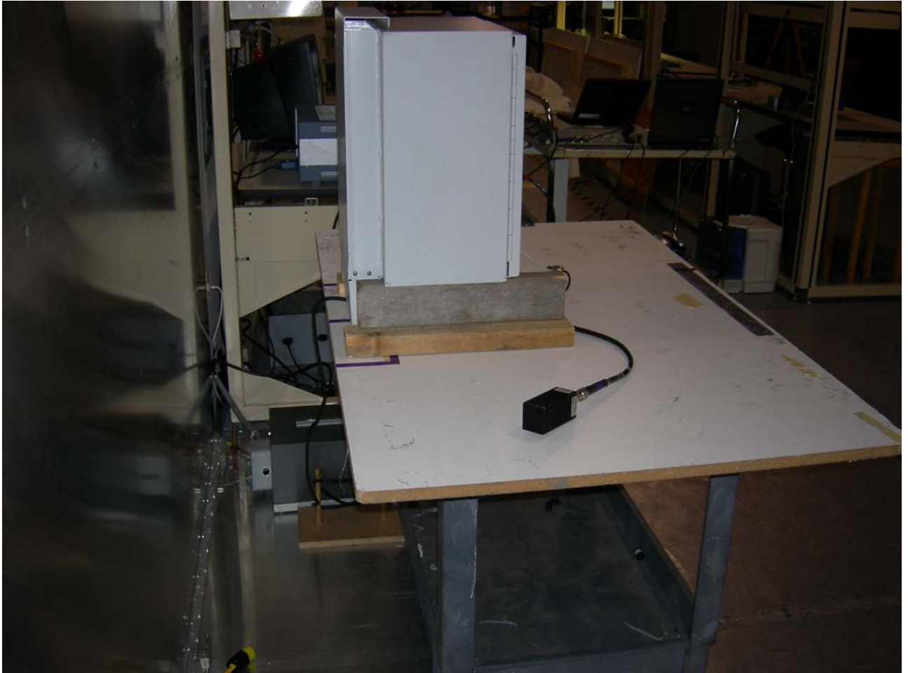
Figure 6: Line Conduction Emissions Rear
