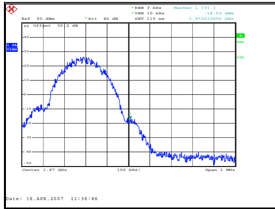
Figure 78: Band-Edge Downlink GSM High Channel
