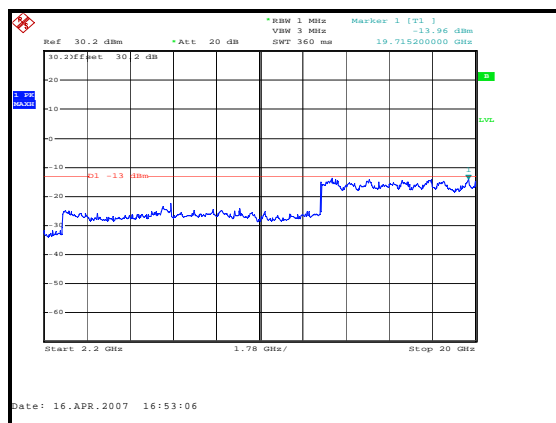
Figure 21: Spurious Emissions - Uplink CDMA Low Channel – Inter-modulation – 2.2 to 20GHz
