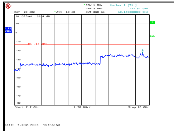
Figure 44: Spurious Emissions - Uplink GSM Mid Channel – 2.2 to 20GHz
