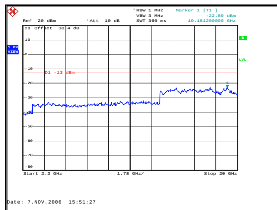
Figure 42: Spurious Emissions - Uplink GSM Low Channel – 2.2 to 20GHz
