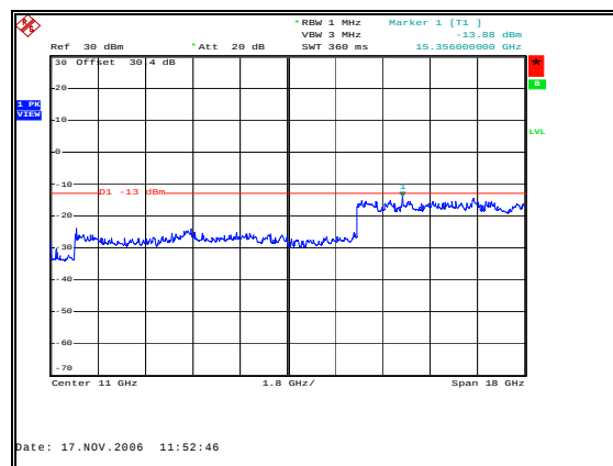
Figure 54: Spurious Emissions - Downlink CDMA High Channel – Inter-modulation - 2.2 to 20GHz
