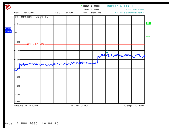
Figure 46: Spurious Emissions - Uplink GSM High Channel – 2.2 to 20GHz
