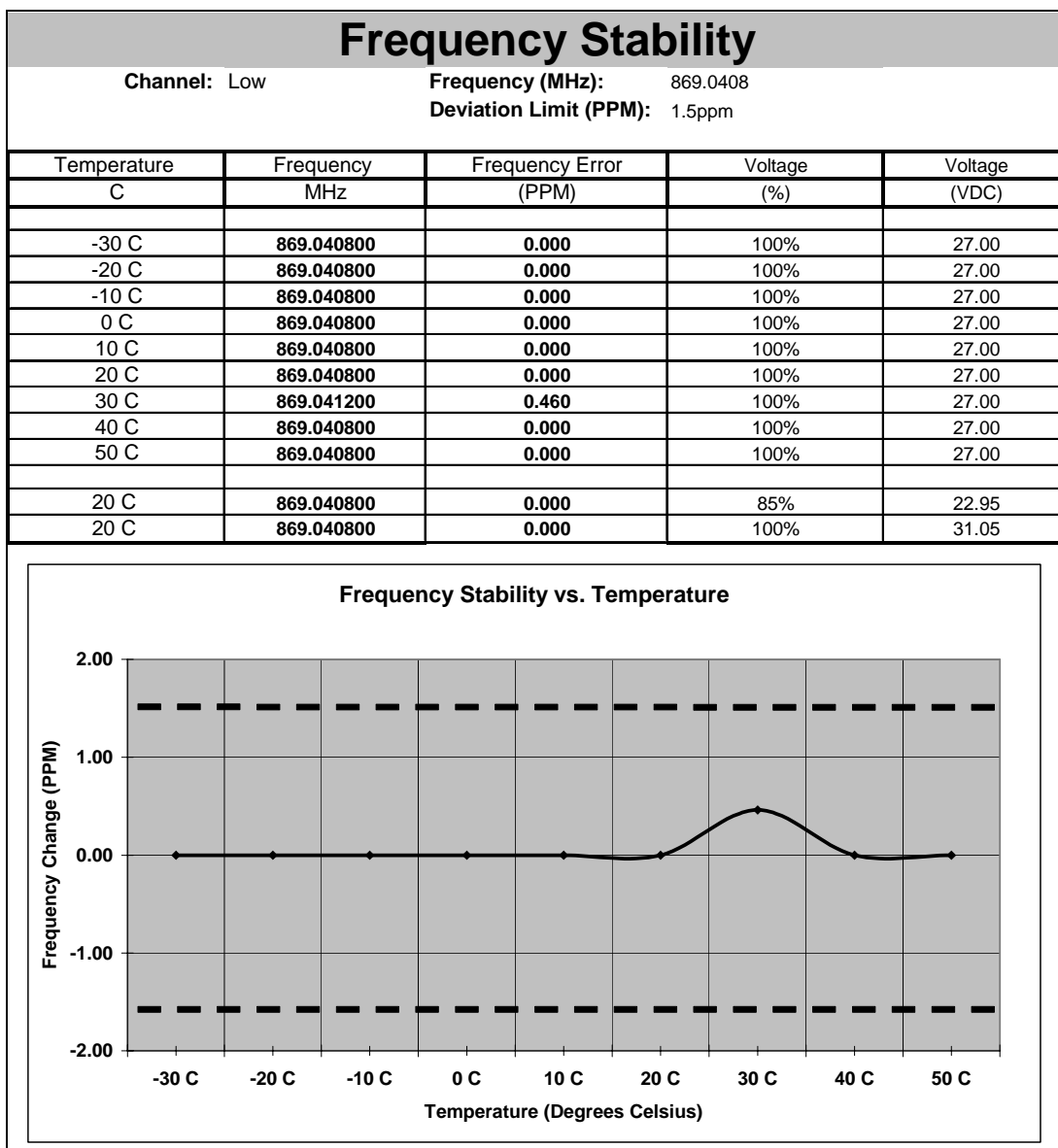
Figure 7.8-4: Frequency Stability Downlink – Low Channel
