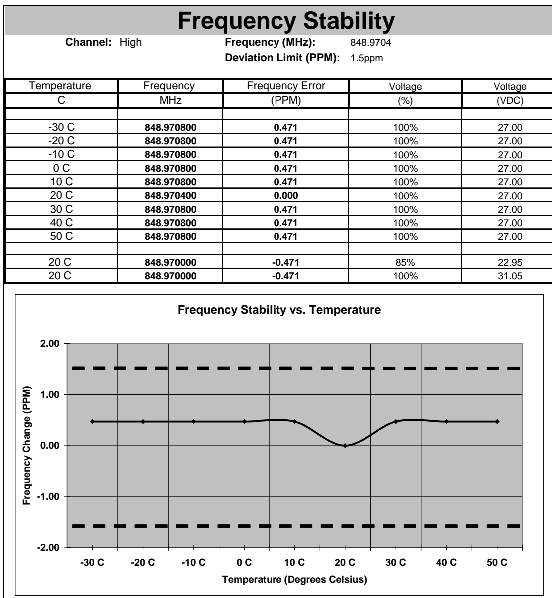
Figure 7.8-3: Frequency Stability Uplink – High Channel
