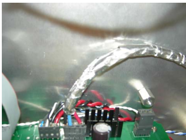
Figure 1.4-3 – Internal Photographs – Foil Wrapped Cable at DC Interconnect PCB
