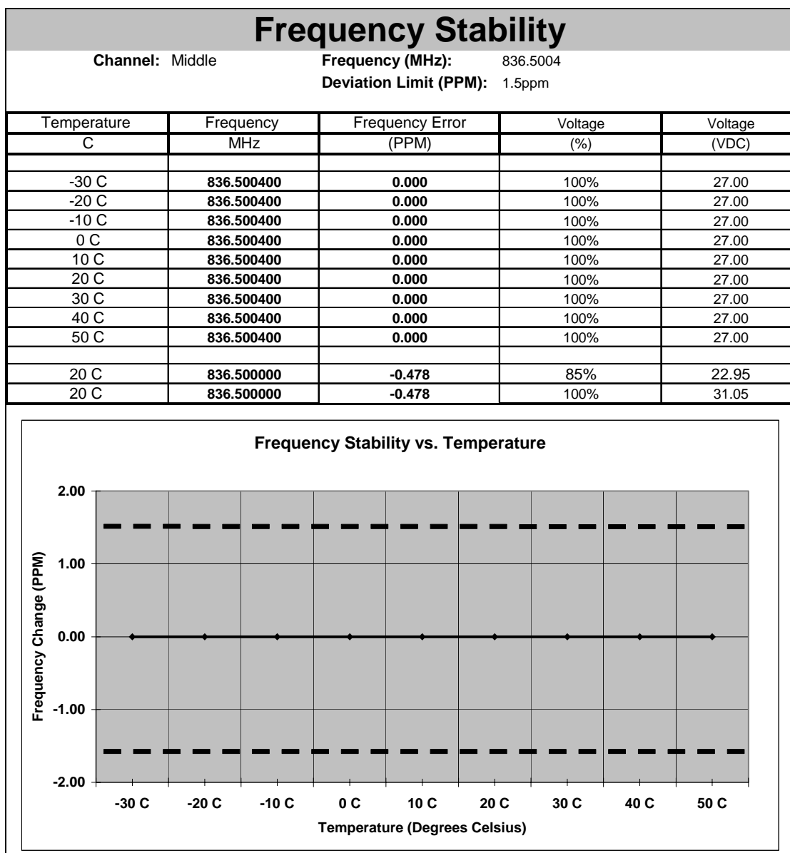
Figure 7.8-2: Frequency Stability Uplink – Middle Channel
