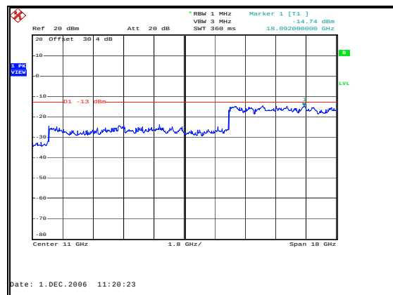
Figure 29: Spurious Emissions - Uplink TDMA Low Channel – Inter-modulation - 2 to 20GHz
