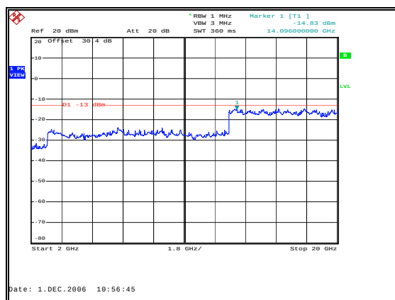
Figure 68: Spurious Emissions - Downlink CW High Channel – Inter-modulation - 2 to 20GHz
