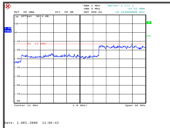
Figure 40: Spurious Emissions - Uplink CW High Channel – Inter-modulation - 2 to 20GHz
