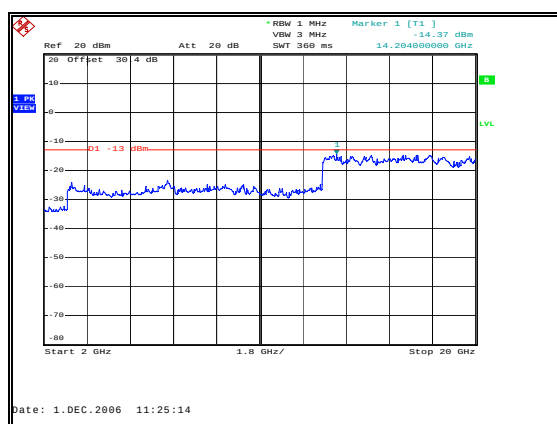
Figure 34: Spurious Emissions - Uplink TDMA High Channel – Inter-modulation - 2 to 20GHz
