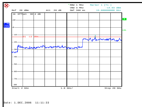
Figure 37: Spurious Emissions - Uplink CW Low Channel – Inter-modulation - 2 to 20GHz
