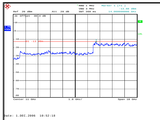
Figure 65: Spurious Emissions - Downlink CW Low Channel – Inter-modulation - 2 to 20GHz
