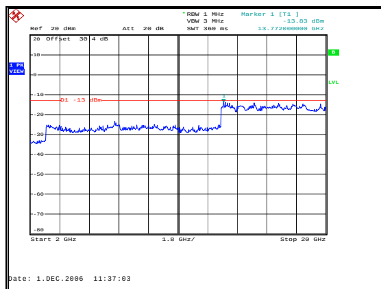
Figure 21: Spurious Emissions - Uplink CDMA Low Channel – Inter-modulation - 2 to 20GHz
