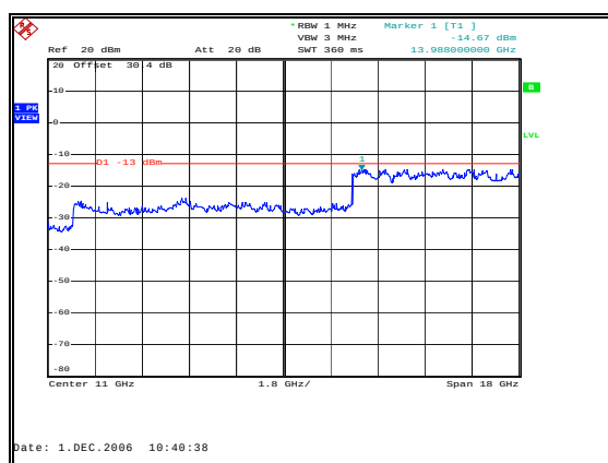
Figure 62: Spurious Emissions - Downlink TDMA High Channel – Inter-modulation - 2 to 20GHz
