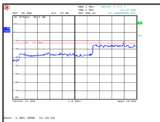
Figure 26: Spurious Emissions - Uplink CDMA High Channel – Inter-modulation - 2 to 20GHz
