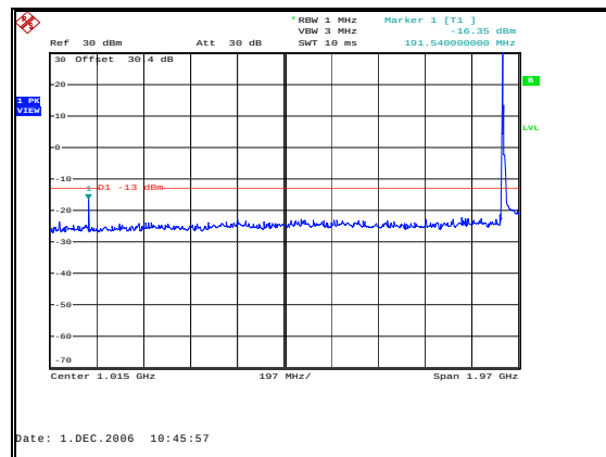
Figure 56: Spurious Emissions - Downlink TDMA Low Channel–Inter-modulation-30MHz to 2GHz
