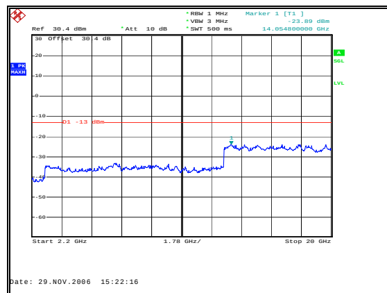
Figure 31: Spurious Emissions - Uplink TDMA Mid Channel – 2.2 to 20GHz
