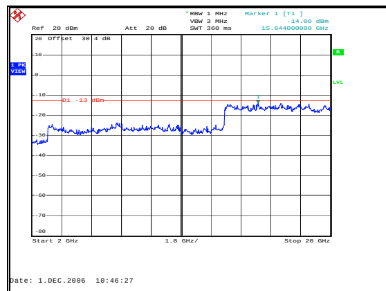
Figure 57: Spurious Emissions - Downlink TDMA Low Channel – Inter-modulation - 2 to 20GHz
