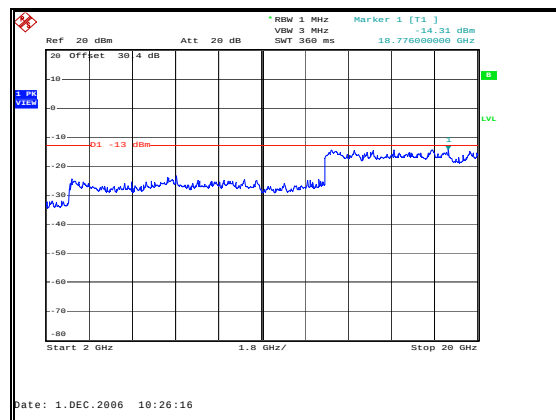
Figure 49: Spurious Emissions - Downlink CDMA Low Channel – Inter-modulation - 2 to 20GHz
