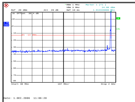
Figure 39: Spurious Emissions - Uplink CW High Channel – Inter-modulation - 30MHz to 2GHz
