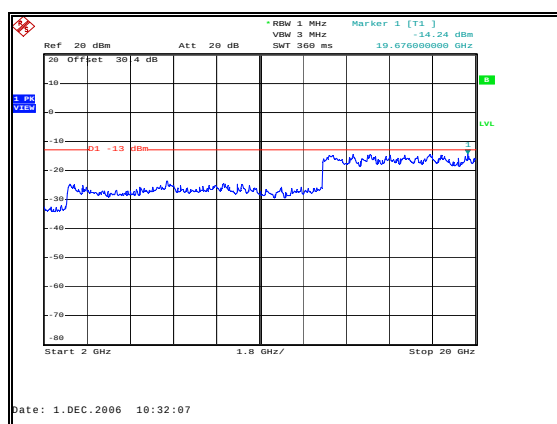
Figure 54: Spurious Emissions - Downlink CDMA High Channel – Inter-modulation - 2 to 20GHz
