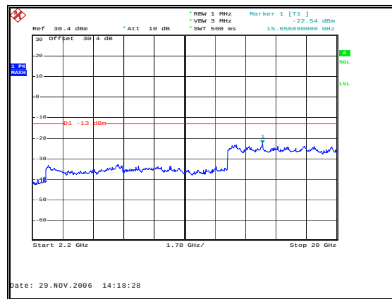
Figure 42: Spurious Emissions - Uplink GSM Low Channel – 2.2 to 20GHz
