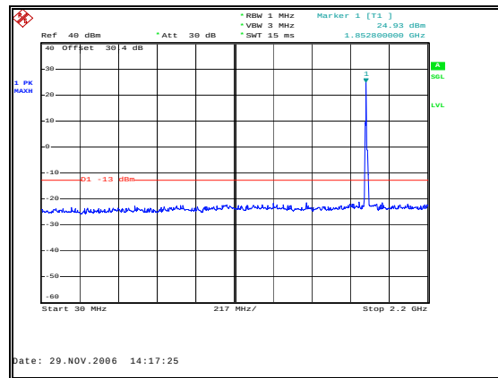
Figure 41: Spurious Emissions - Uplink GSM Low Channel – 30MHz to 2.2GHz
