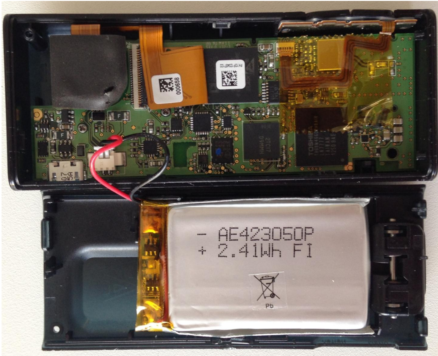
Internal Assemblies View
