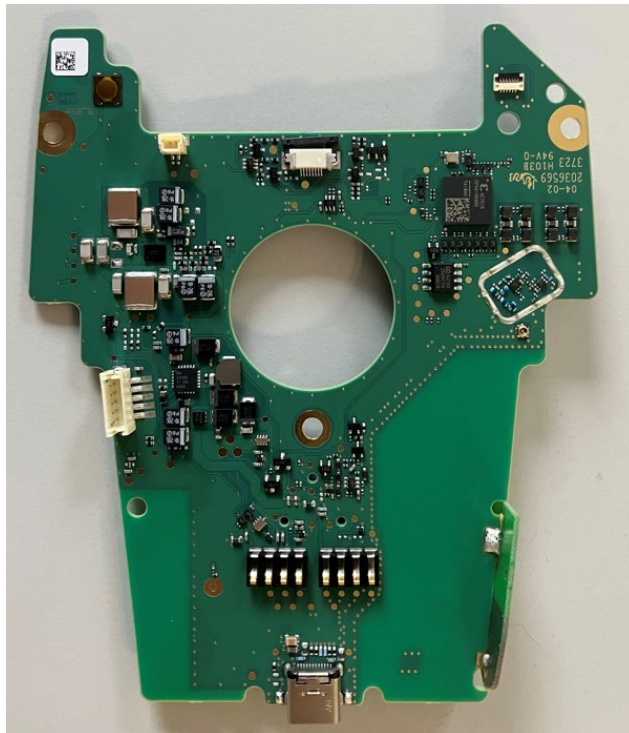
Top View (Main PCB)
