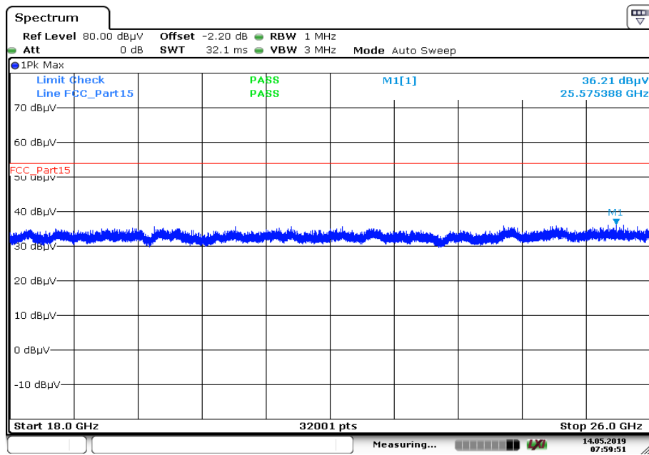
Plot 10: 18 GHz to 26 GHz, TX mode, 2443 MHz, vertical & horizontal polarization, antenna 2
