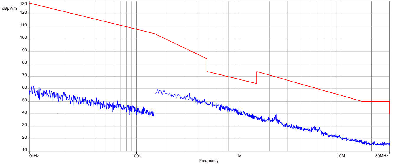
Plot 1: 9 kHz to 30 MHz, 2403 MHz, transmit mode, Antenna 1
