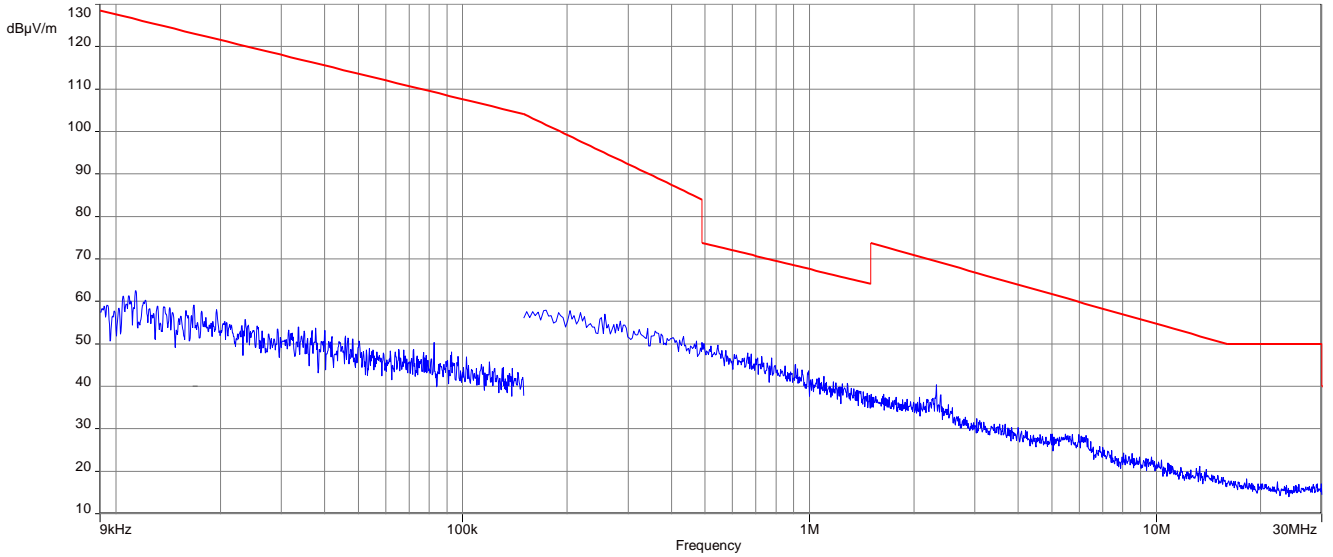
Plot 3: 9 kHz to 30 MHz, 2481 MHz, transmit mode, Antenna 1
