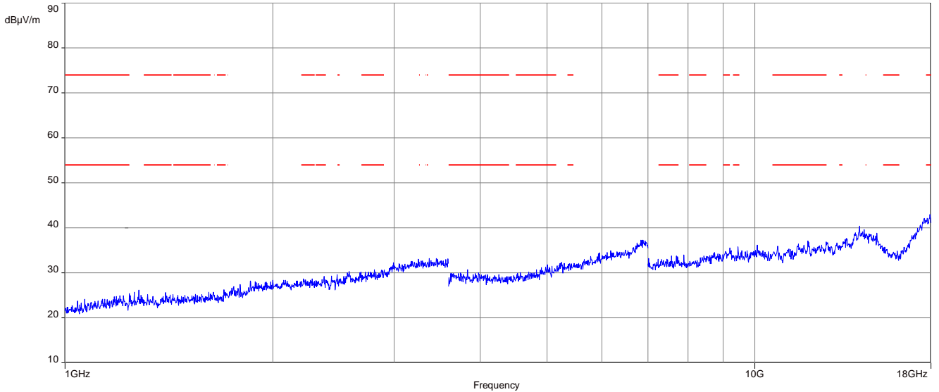
Plot 5: 1 GHz to 18 GHz, TX mode, 2481 MHz, vertical & horizontal polarization, antenna 1
