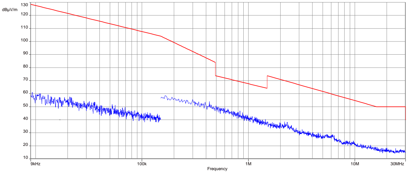
Plot 4: 9 kHz to 30 MHz, 2403 MHz, transmit mode, Antenna 2
