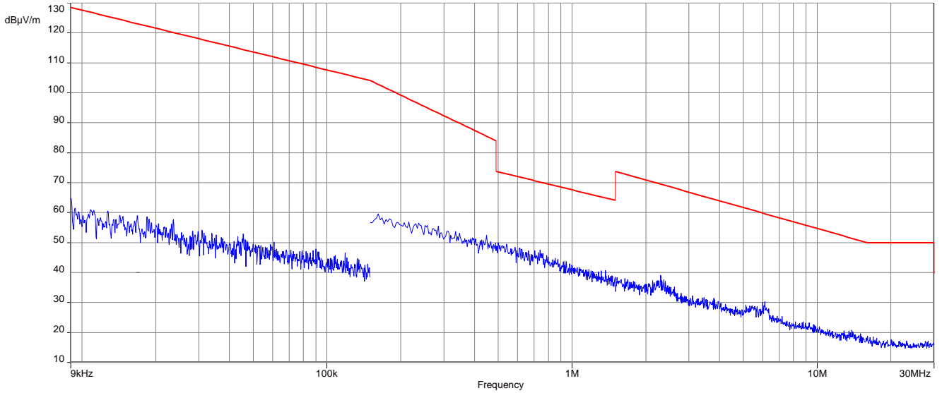
Plot 5: 9 kHz to 30 MHz, 2443 MHz, transmit mode, Antenna 2
