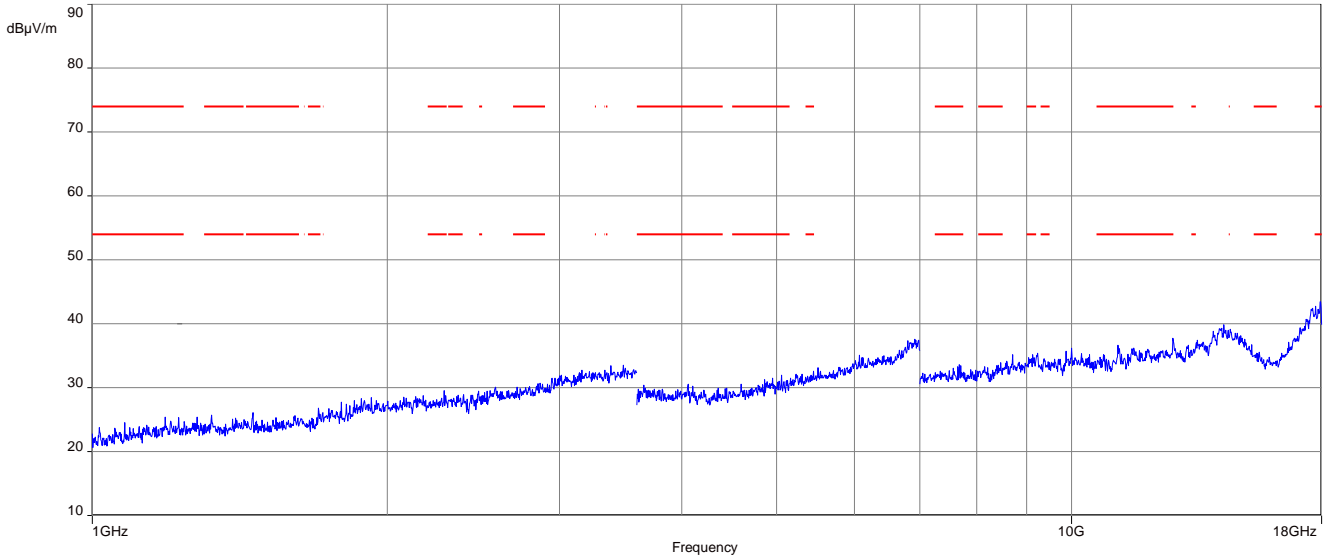
Plot 3: 1 GHz to 18 GHz, TX mode, 2443 MHz, vertical & horizontal polarization, antenna 1
