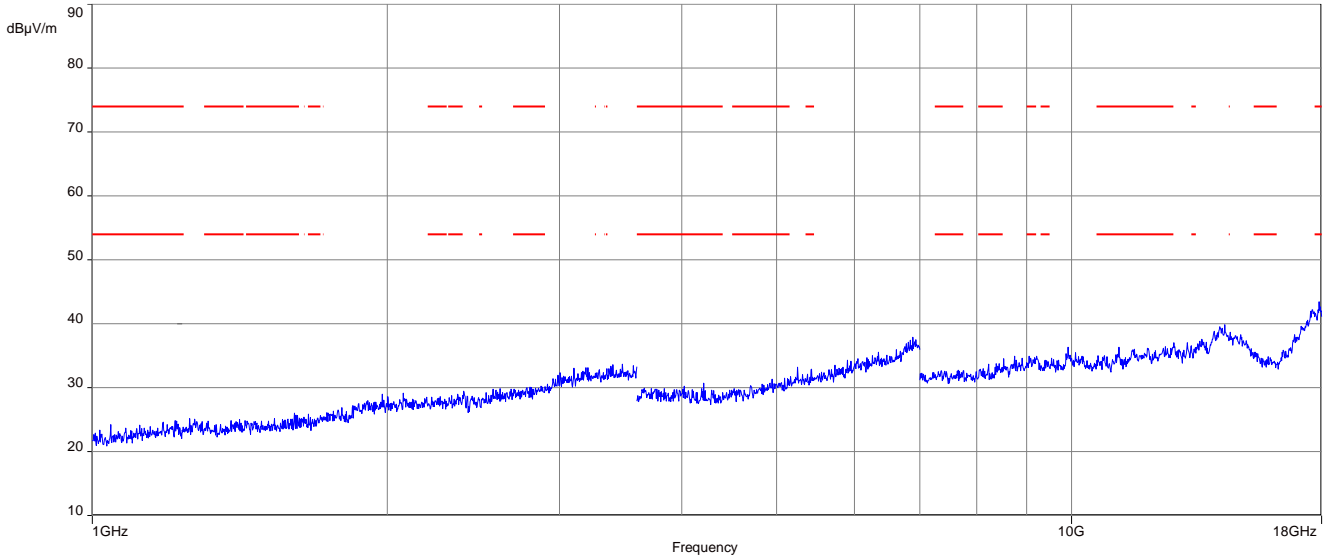
Plot 9: 1 GHz to 18 GHz, TX mode, 2443 MHz, vertical & horizontal polarization, antenna 2
