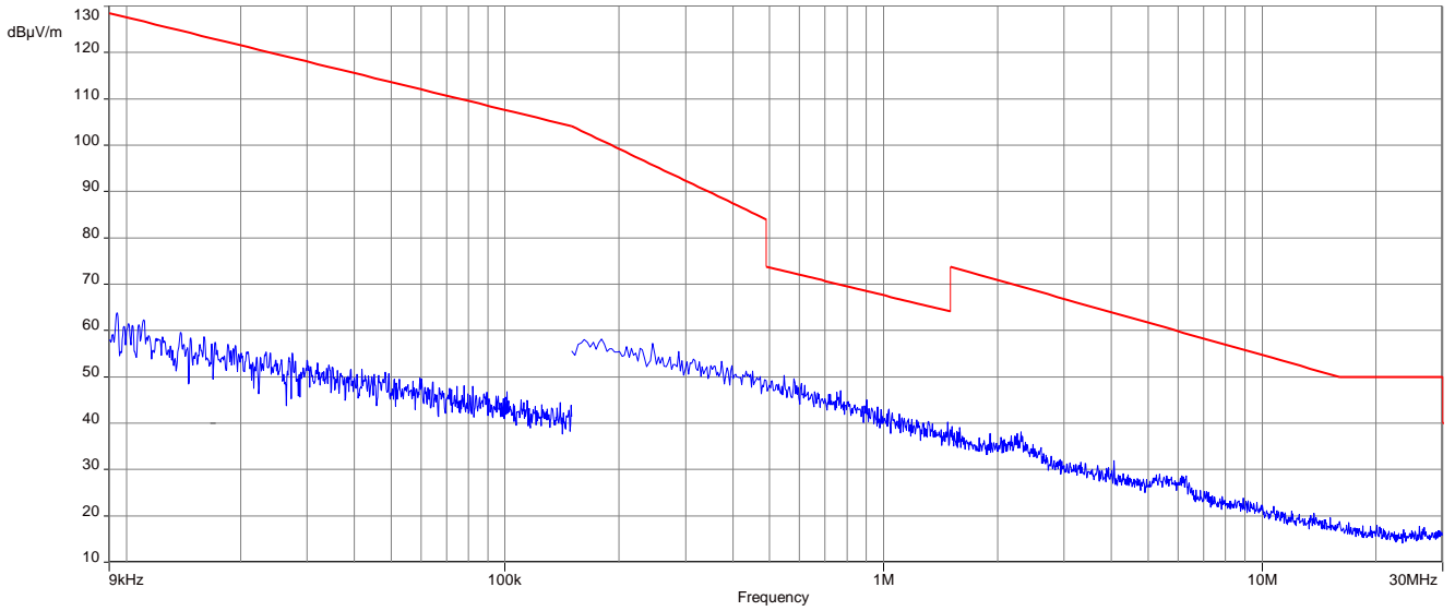
Plot 2: 9 kHz to 30 MHz, 2443 MHz, transmit mode, Antenna 1
