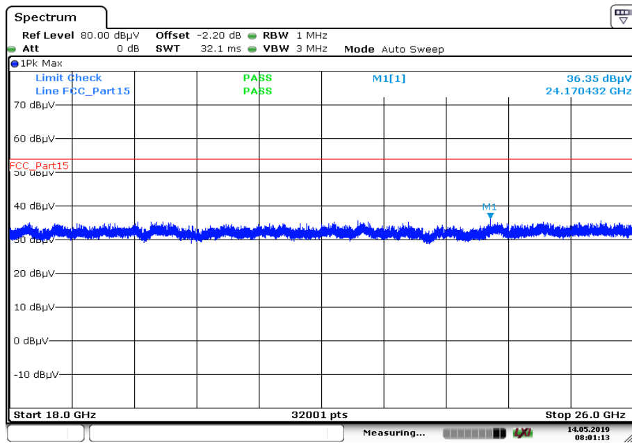
Plot 12: 18 GHz to 26 GHz, TX mode, 2481 MHz, vertical & horizontal polarization, antenna 2
