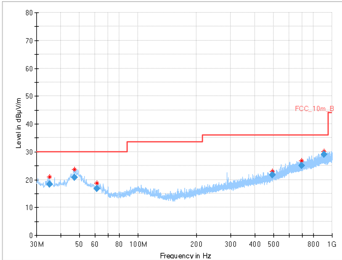
Plot 6: 30 MHz to 1 GHz, TX mode, 2481 MHz, vertical & horizontal polarization, antenna 2
