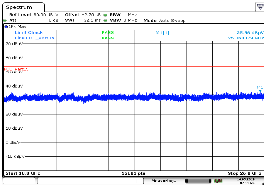
Plot 2: 18 GHz to 26 GHz, RX / idle – mode, vertical & horizontal polarization, antenna 1
