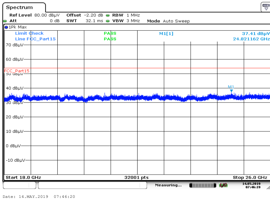
Plot 4: 18 GHz to 26 GHz, RX / idle – mode, vertical & horizontal polarization, antenna 2
