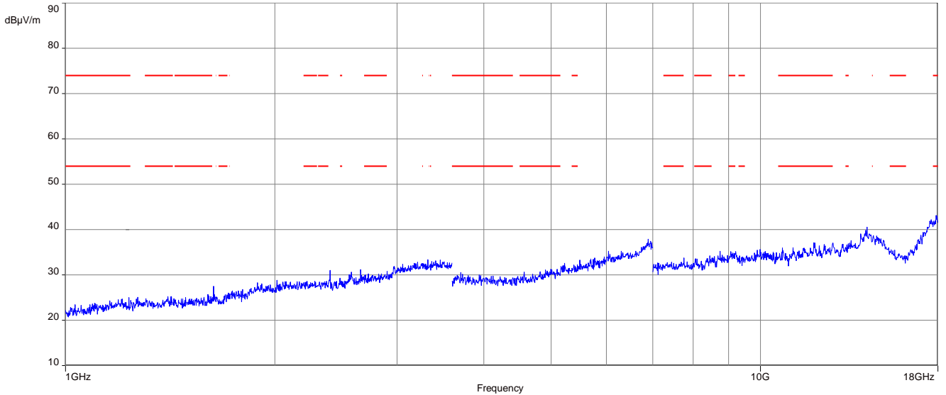
Plot 7: 1 GHz to 18 GHz, TX mode, 2403 MHz, vertical & horizontal polarization, Antenna 2
