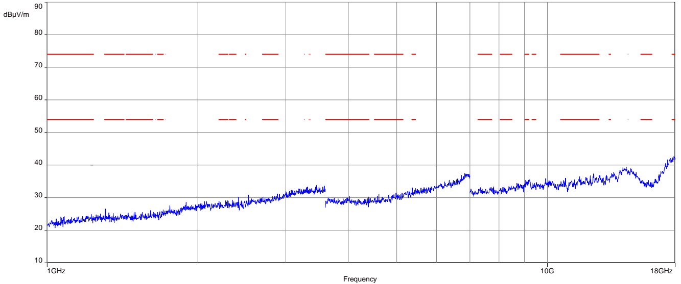
Plot 11: 1 GHz to 18 GHz, TX mode, 2481 MHz, vertical & horizontal polarization, antenna 2
