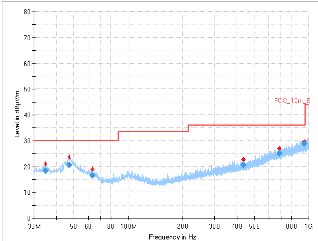
Plot 5: 30 MHz to 1 GHz, TX mode, 2443 MHz, vertical & horizontal polarization, antenna 2
