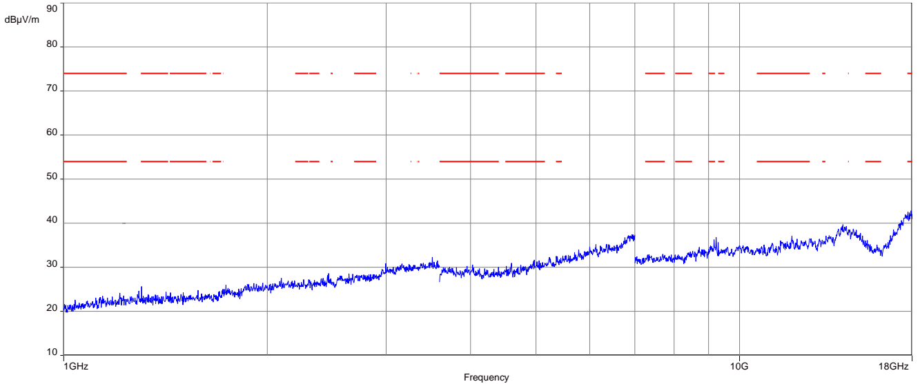
Plot 1: 1 GHz to 18 GHz, RX / idle – mode, vertical & horizontal polarization, antenna 1
