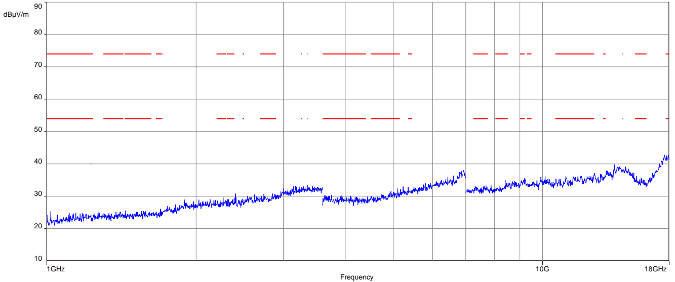
Plot 1: 1 GHz to 18 GHz, TX mode, 2403 MHz, vertical & horizontal polarization, antenna 1
