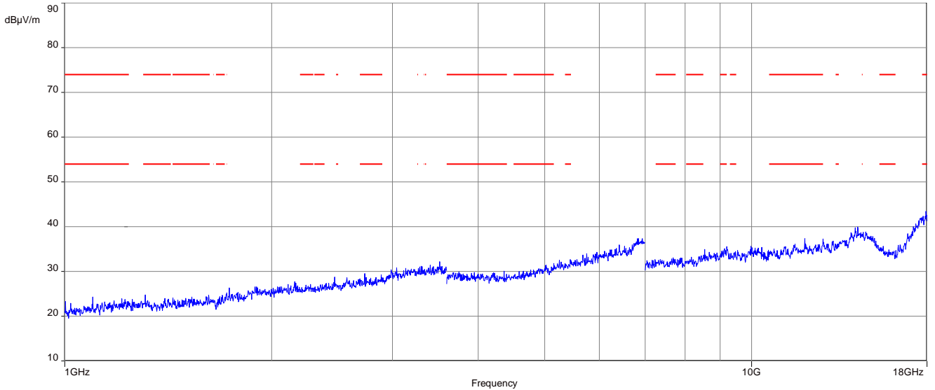
Plot 3: 1 GHz to 18 GHz, RX / idle – mode, vertical & horizontal polarization, antenna 2
