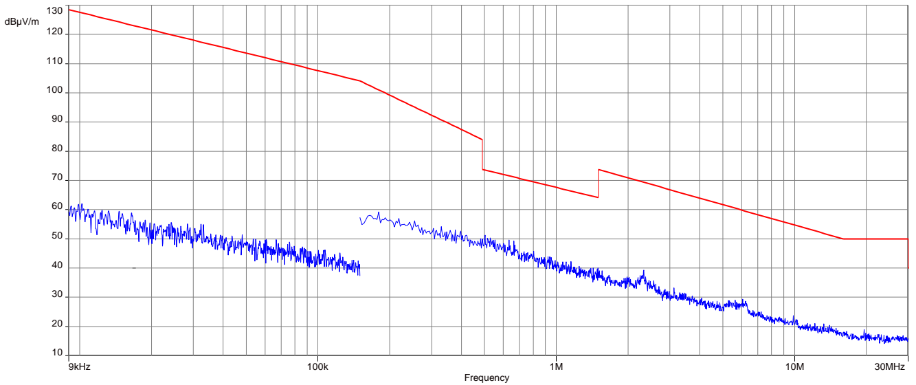
Plot 6: 9 kHz to 30 MHz, 2481 MHz, transmit mode, Antenna 2
