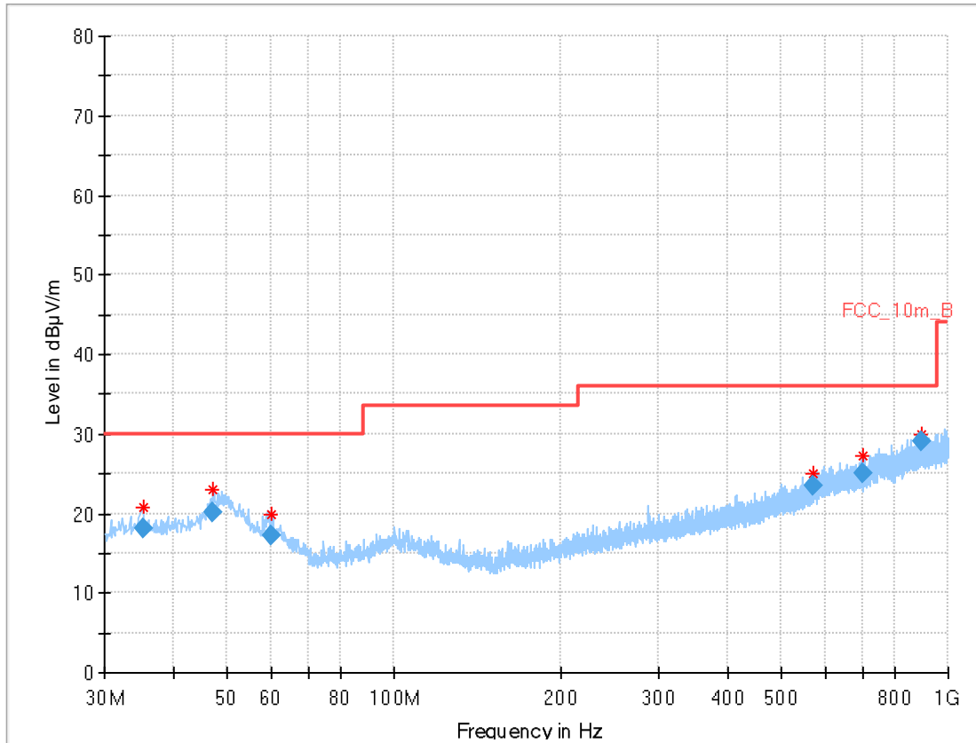
Plot 2: 30 MHz to 1 GHz, RX / idle – mode, vertical & horizontal polarization, antenna 2
