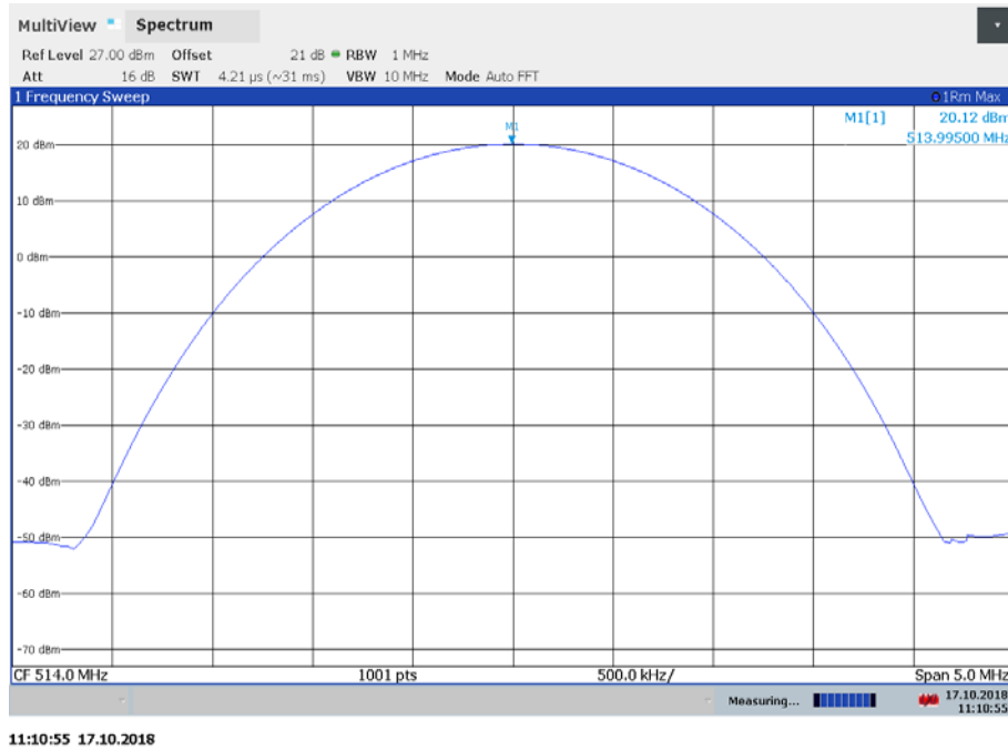
Plot 3: 514 MHz, average (modulated carrier)
