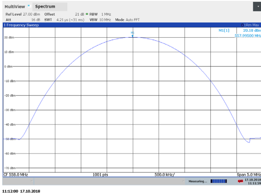
Plot 5: 558 MHz, average (modulated carrier)
