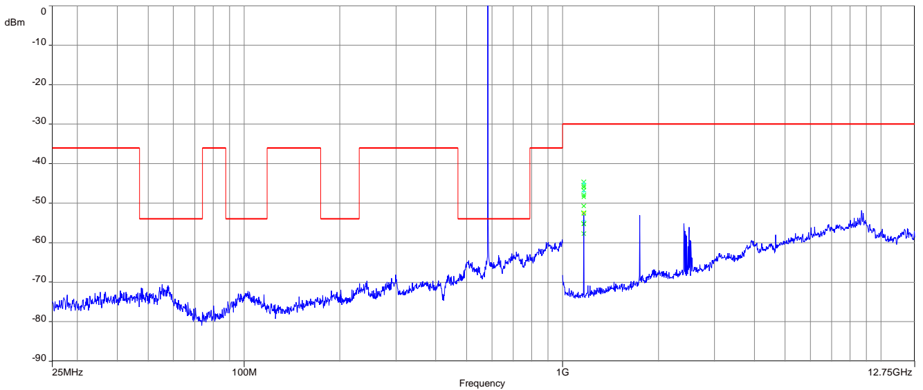
Plot 2: 583.0 MHz, spurious emissions, 25 MHz – 12.75 GHz
