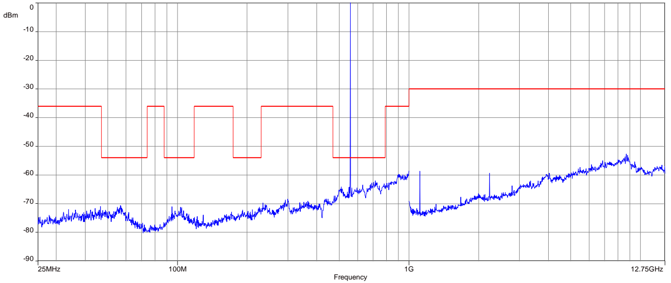
Plot 1: 558.0 MHz, spurious emissions, 25 MHz – 12.75 GHz
