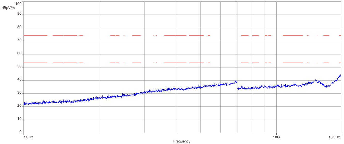
Plot 1: 1 GHz to 18 GHz, RX / idle – mode, vertical & horizontal polarization, 1 Msps
