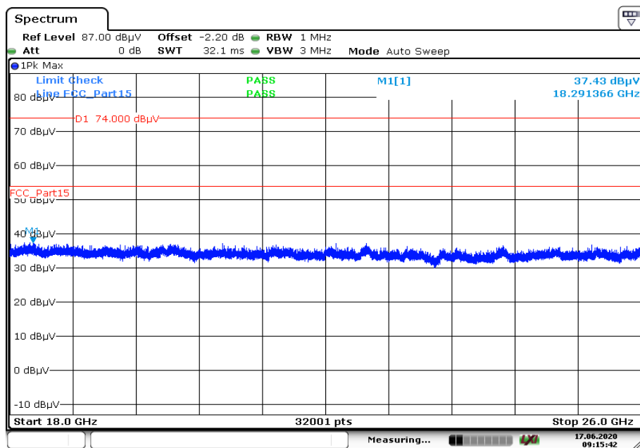
Plot 2: 18 GHz to 26 GHz, RX / idle – mode, vertical & horizontal polarization, 1 Msps
