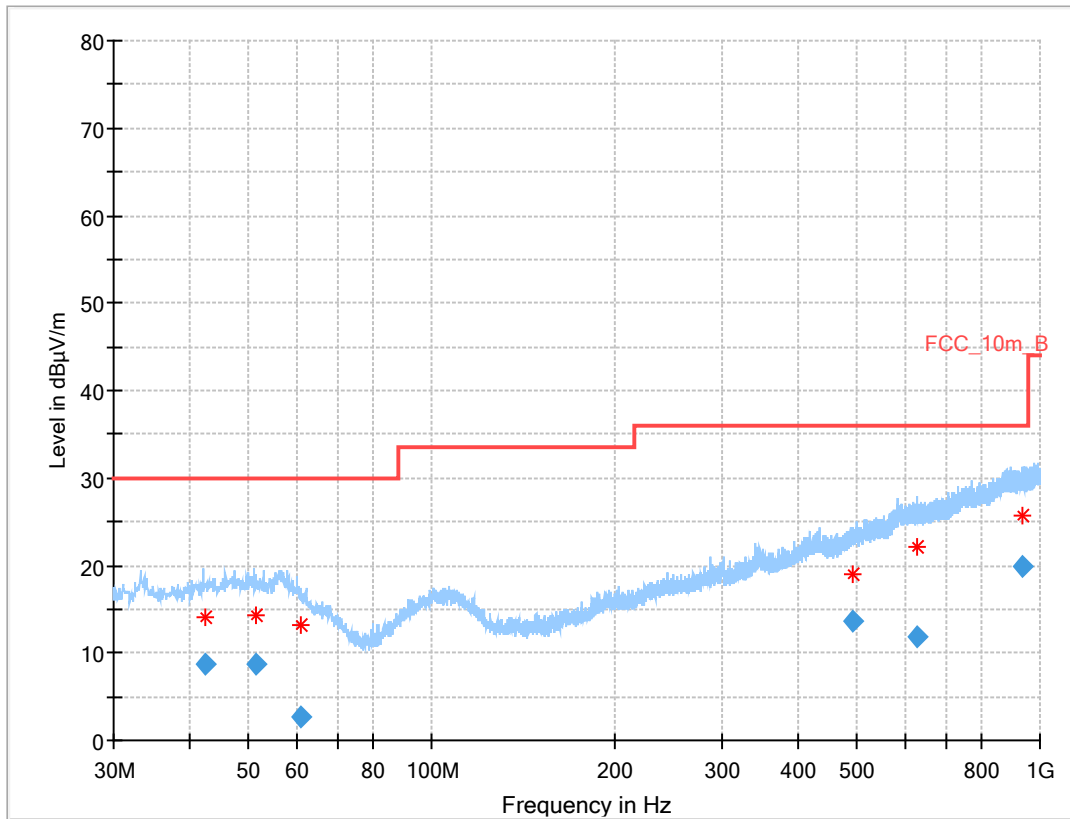
Plot 2: 30 MHz to 1 GHz, RX / idle – mode, vertical & horizontal polarization, 2 Msps
