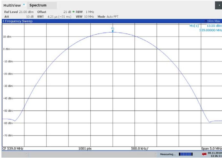
Plot 1: middle channel, average (modulated carrier)
