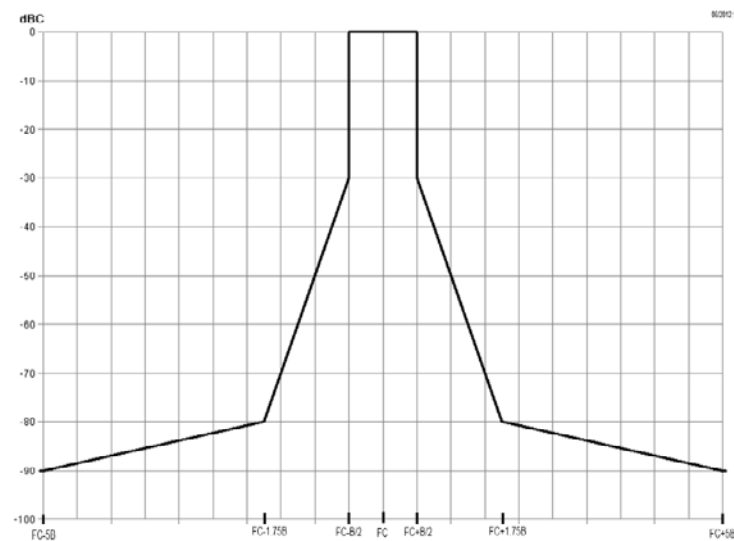
Figure 1: Spectrum mask for digital systems below 2 GHz
