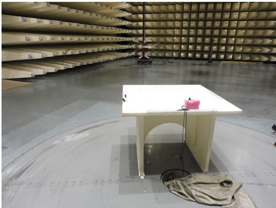
Photo 4: RSE set-up (30MHz to 1GHz)
