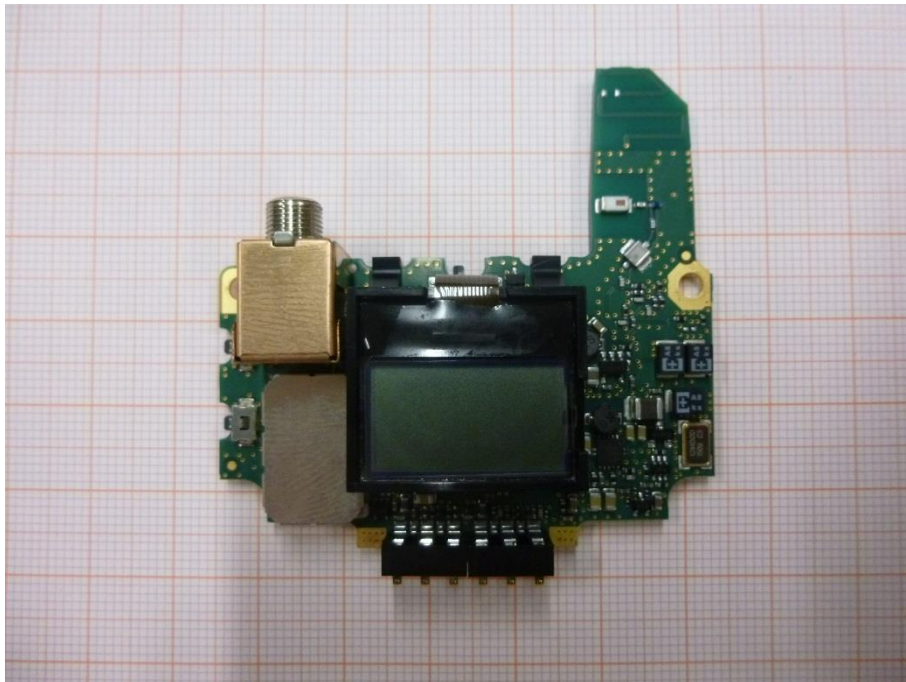
Photo 6: PCB (detailed front view)
