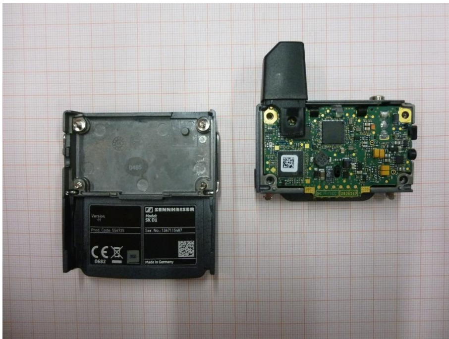
Photo 2: EUT disassembled
