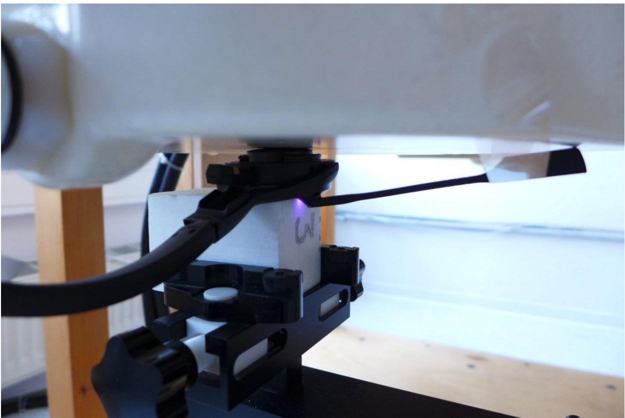
Pic. 4: Test position – inner side, 0 mm distance to phantom, antenna 1 and 2
