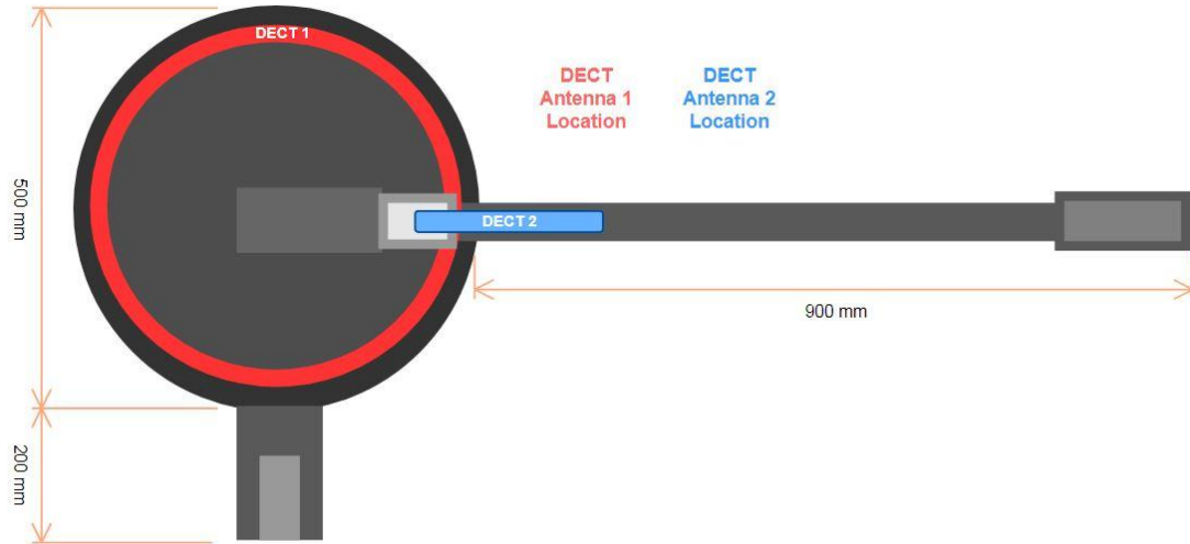
Fig. 1: Sketches and antenna location of the EUT (marked in red).
