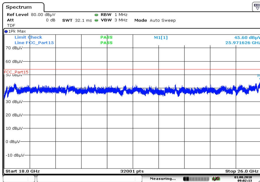
Plot 8: 18 GHz to 26 GHz, TX mode, 2403 MHz, vertical & horizontal polarization, Antenna 2
