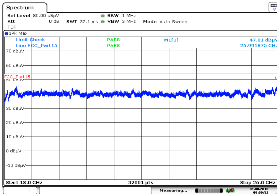
Plot 2: 18 GHz to 26 GHz, TX mode, 2403 MHz, vertical & horizontal polarization, Antenna 1
