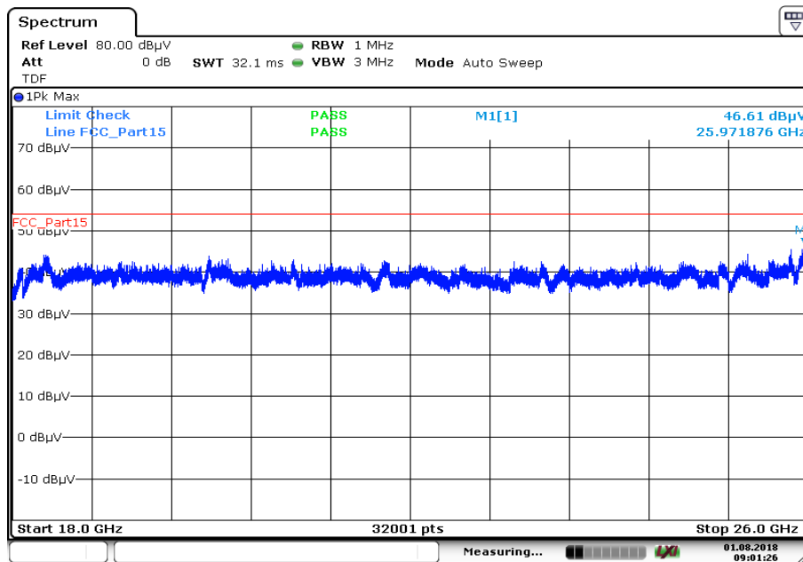
Plot 4: 18 GHz to 26 GHz, TX mode, 2443 MHz, vertical & horizontal polarization, Antenna 1
