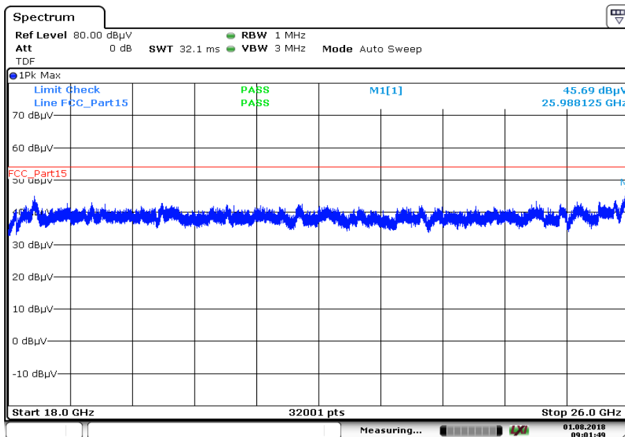
Plot 6: 18 GHz to 26 GHz, TX mode, 2481 MHz, vertical & horizontal polarization, Antenna 1
