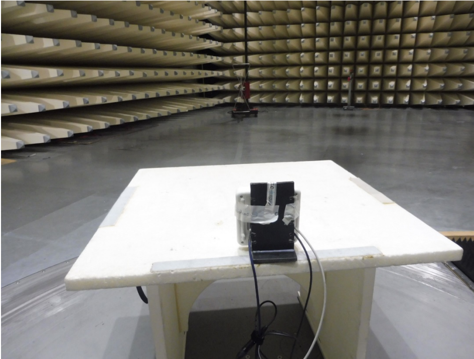
Photo 2: Radiated Emission
