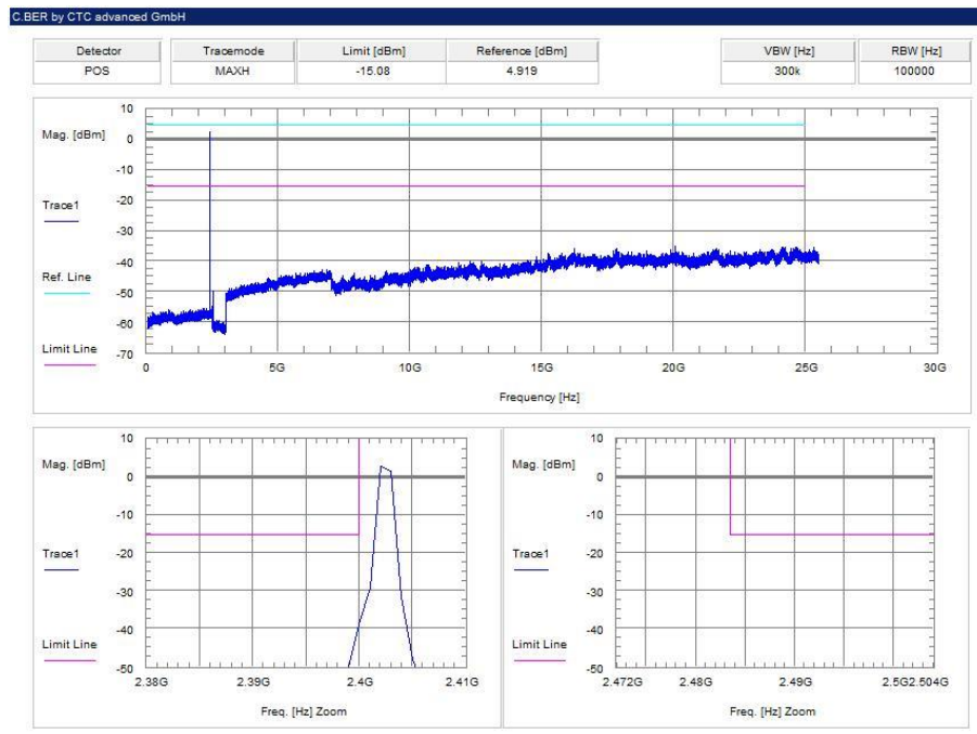
Plot 4: lowest channel – 2402 MHz, Pi/4-DQPSK modulation
