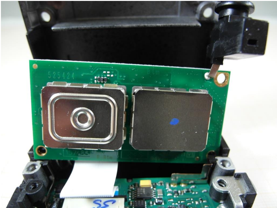
Photo 2: front with shielding and antenna
