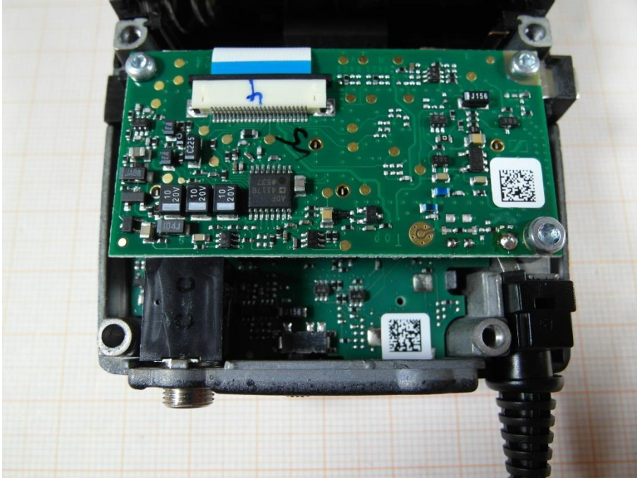
Photo 1: backside RF part
