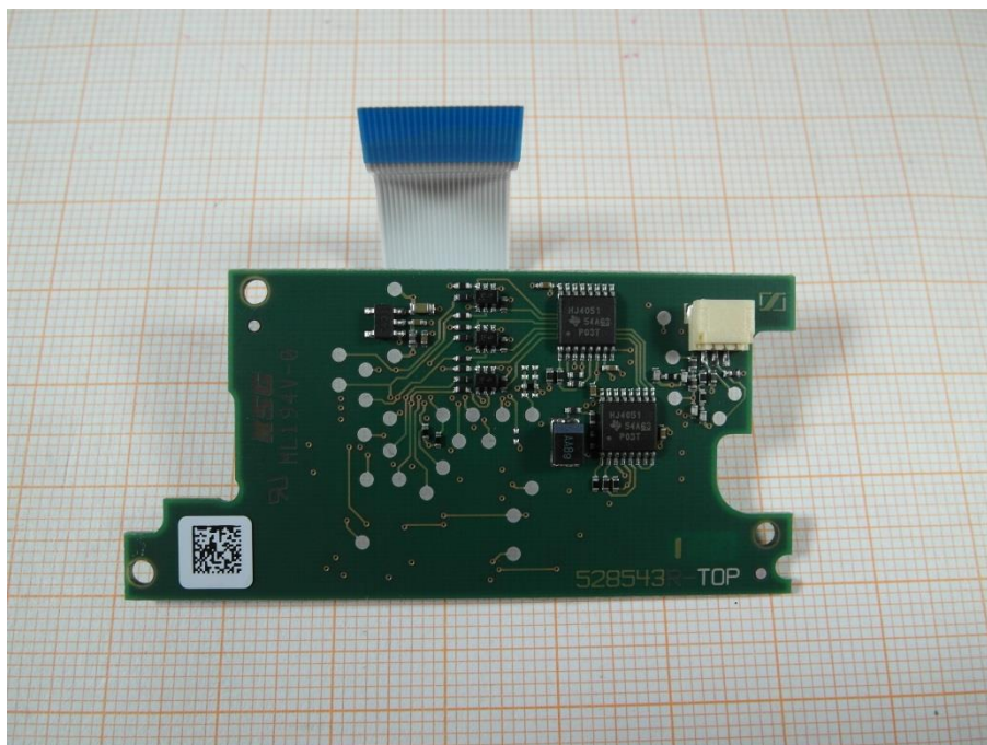
Photo 3: audio part backside
