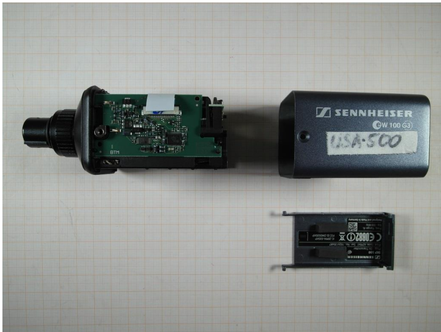
Photo 1: RF part without housing
