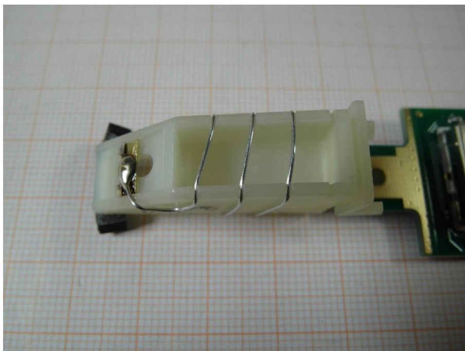
Photo 10: antenna
