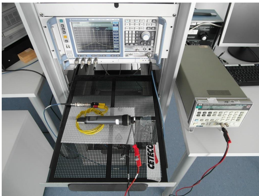
Photo 10: spectrum analyzer
