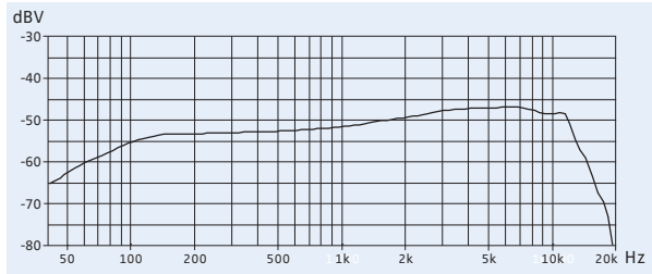
Frequency response curve MMD 935-1
