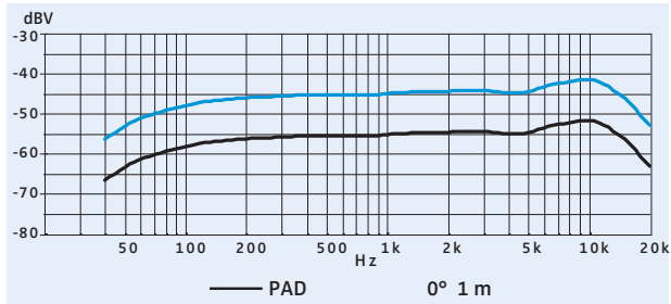
Frequency response curve MMK 965-1 (super-cardioid)
