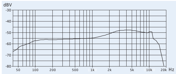
Frequency response curve MMD 945-1
