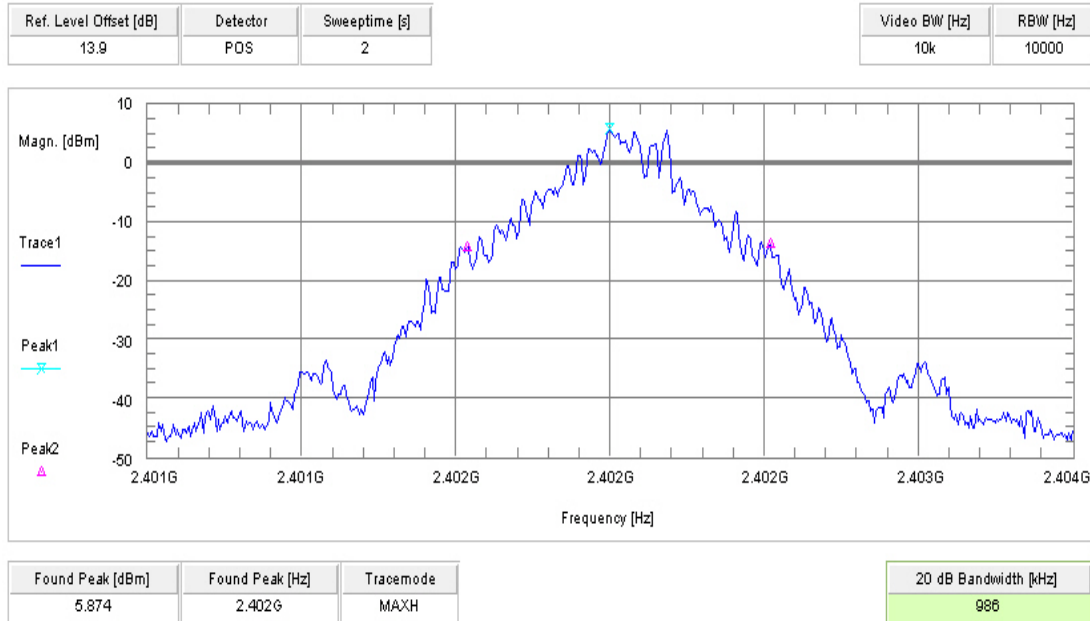
Plot 1 GFSK
