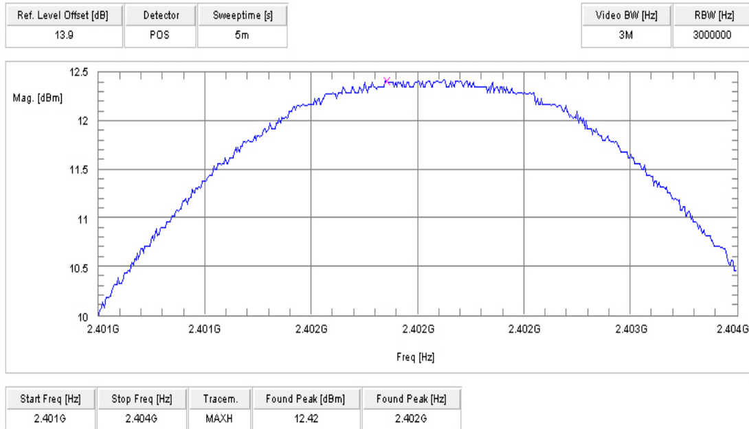
Plot 1 GFSK
