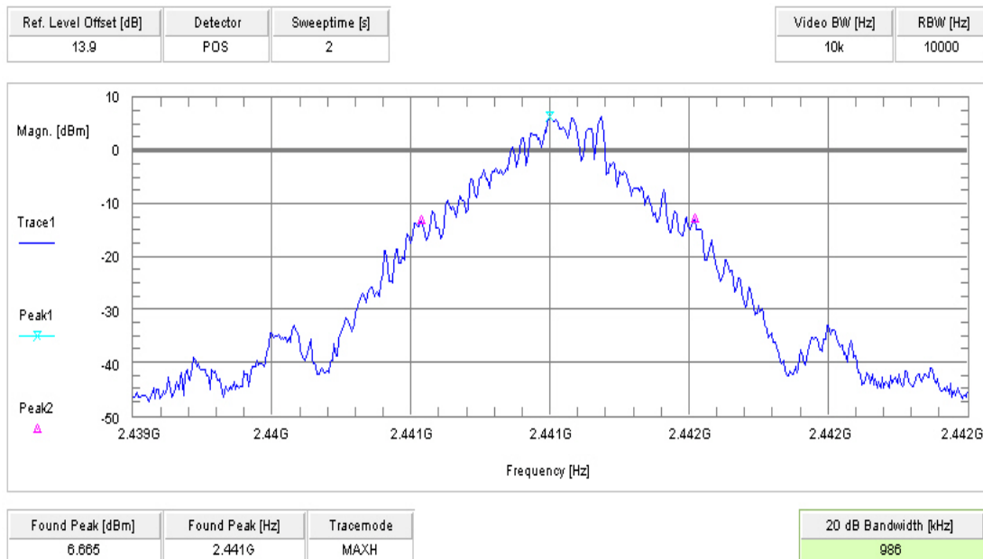
Plot 2 GFSK
