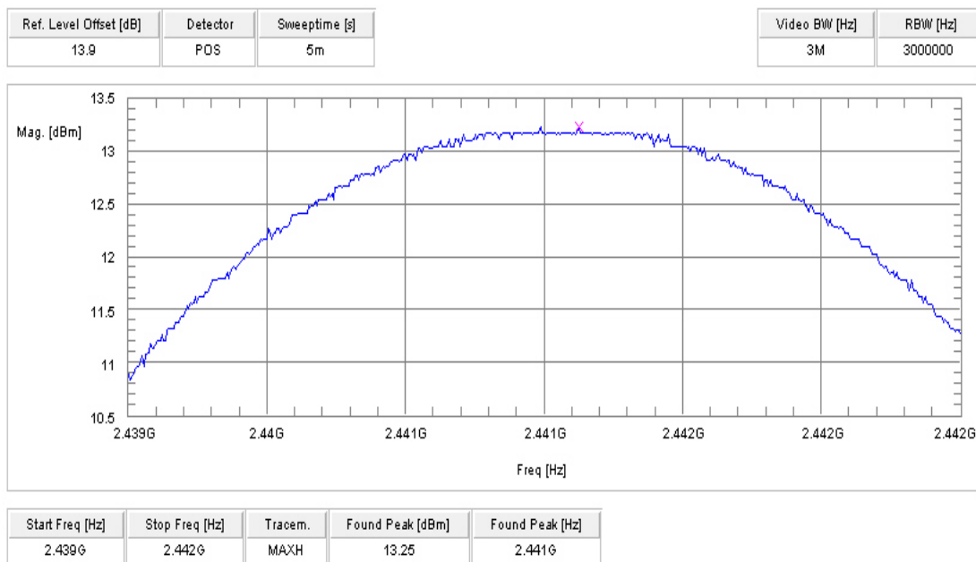
Plot 2 GFSK
