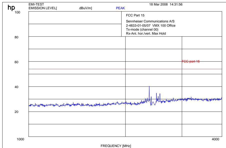
Plot: 1 - 4 GHz vertical worst case (lowest channel)
