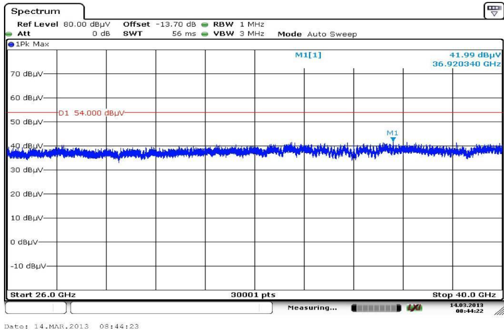
Plot 5: Middle channel, 26 GHz to 40 GHz, vertical & horizontal polarization
