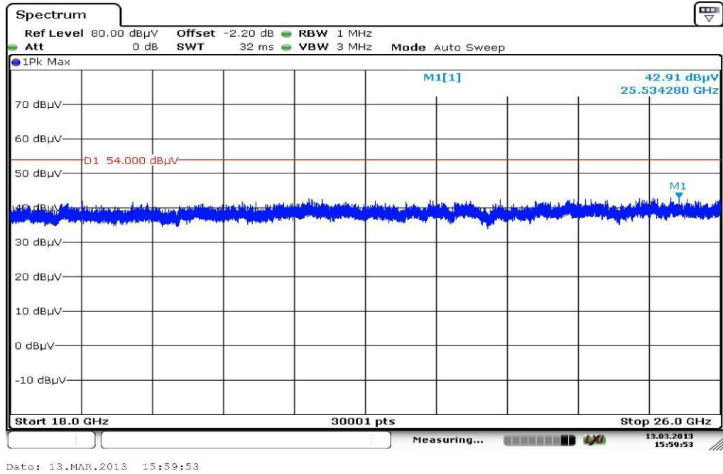
Plot 4: Middle channel, 18 GHz to 26 GHz, vertical & horizontal polarization
