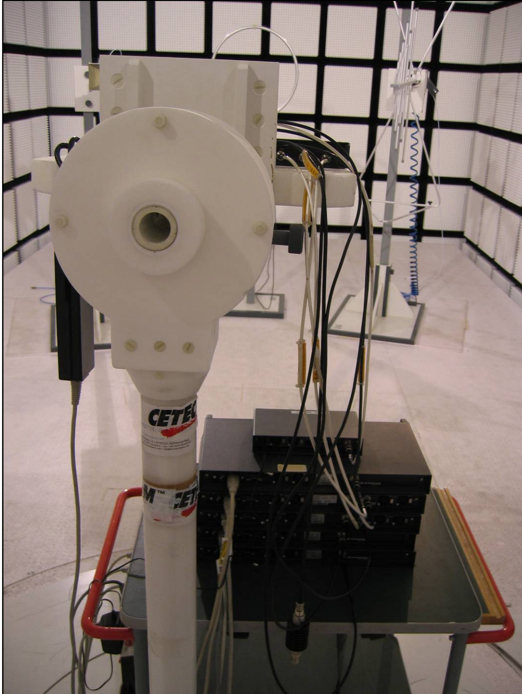
Photo 4: Transmitter measurement
