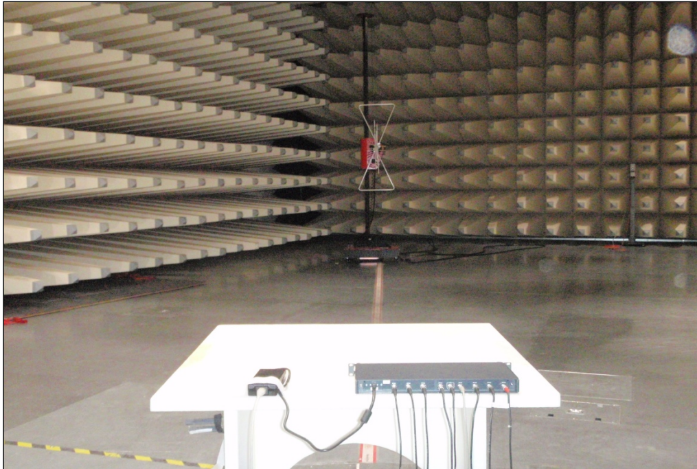
Photo 1: Idle measurement
