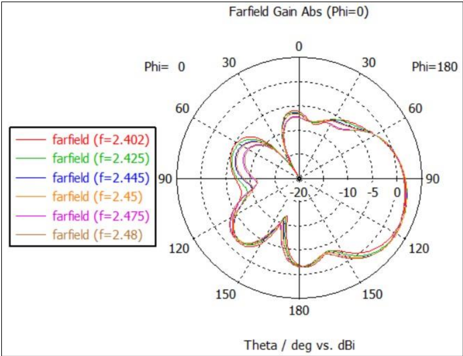
Figure 6: Excitation [1] _Phi=0_farfield cuts (f=2.402, 2.45, and 2.480 GHz)
