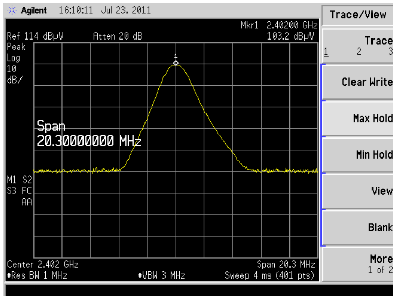
Figure 1 – 199; PRBS 9 GFSK
