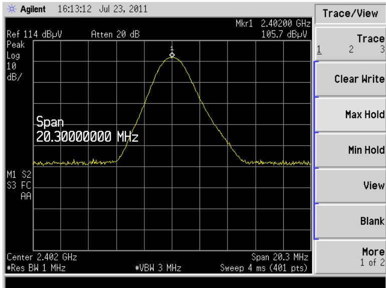
Figure 6 - 204; PRBS 15 8PSK
