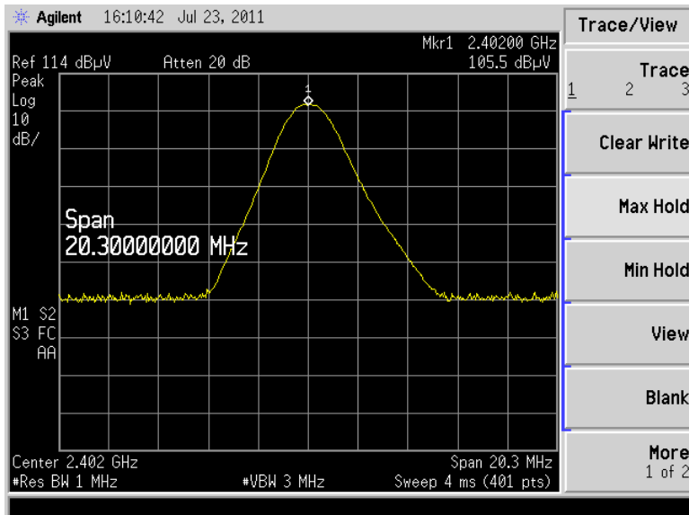
Figure 2 – 200; PRBS 9 QPSK
