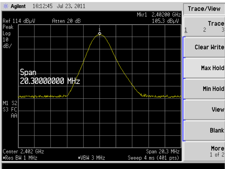
Figure 5 – 203; PRBS 15 QPSK
