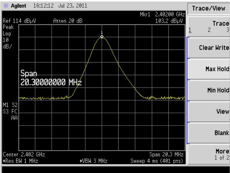
Figure 4 – 202; PRBS 15 GFSK
