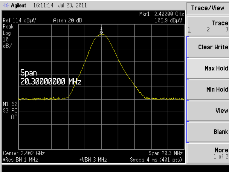
Figure 3 – 201; PRBS 9 8PSK
