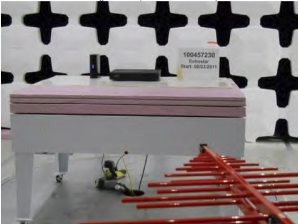
BiLog Antenna (30MHz to 1000MHz)
