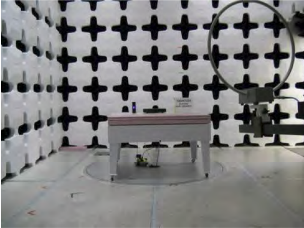
Active Loop Antenna (9kHz to 30MHz)
