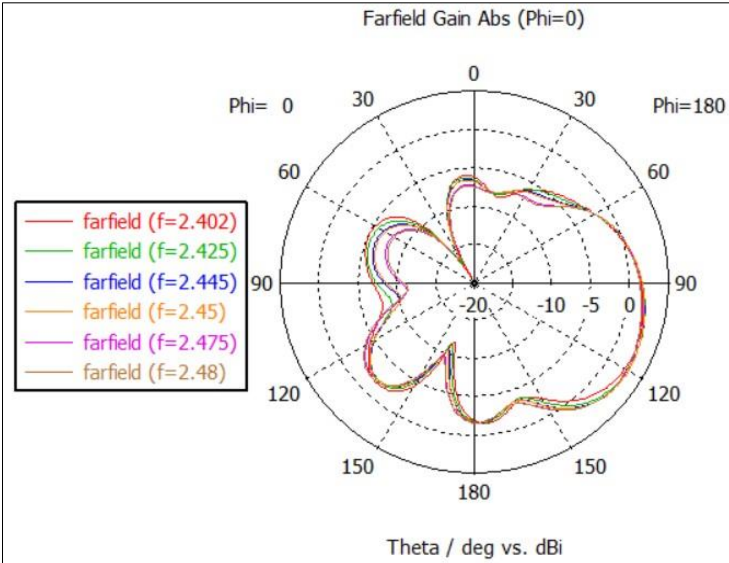
Figure 6: Excitation [1] _Phi=0_farfield cuts (f=2.402, 2.45, and 2.480 GHz)
