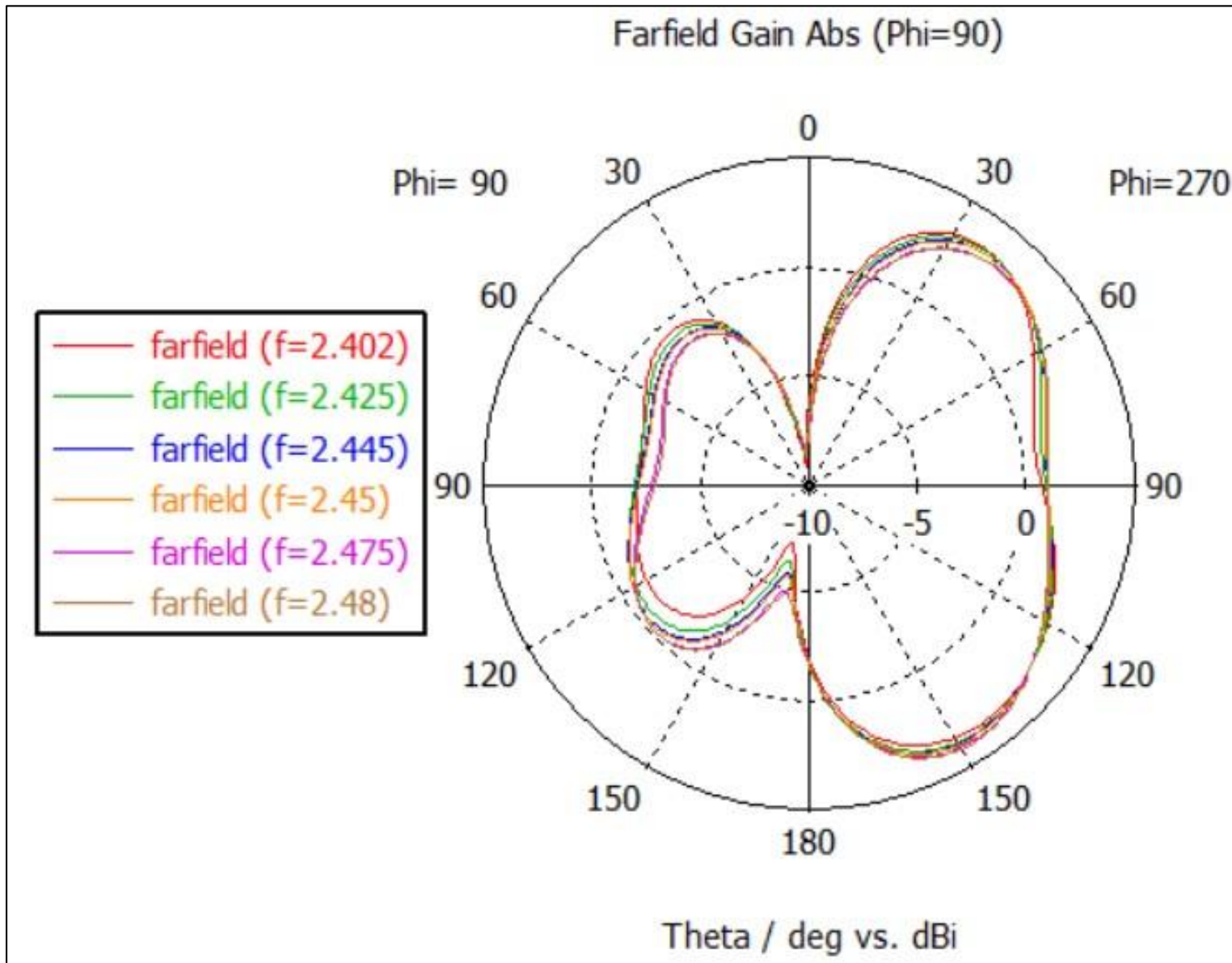
Figure 7: Excitation [1]_Phi=90_farfield cuts (f=2.402, 2.45, and 2.480 GHz)
