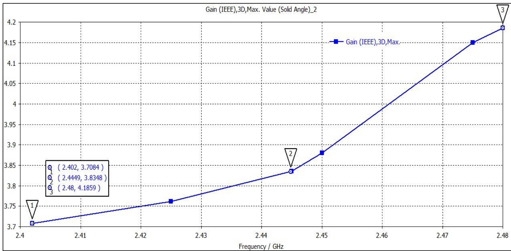
Figure 3: BT/BLE Max simulated Antenna Gain
