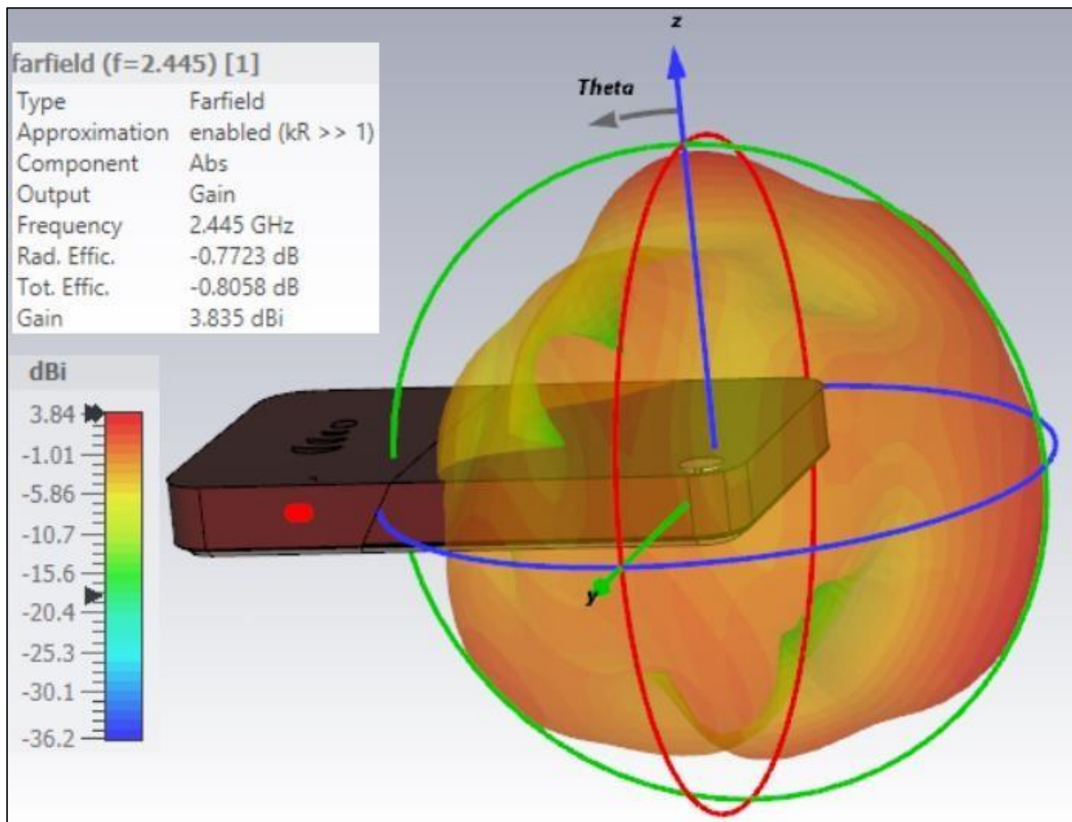
Figure 4: Farfield radiation pattern at 2.445 GHz
