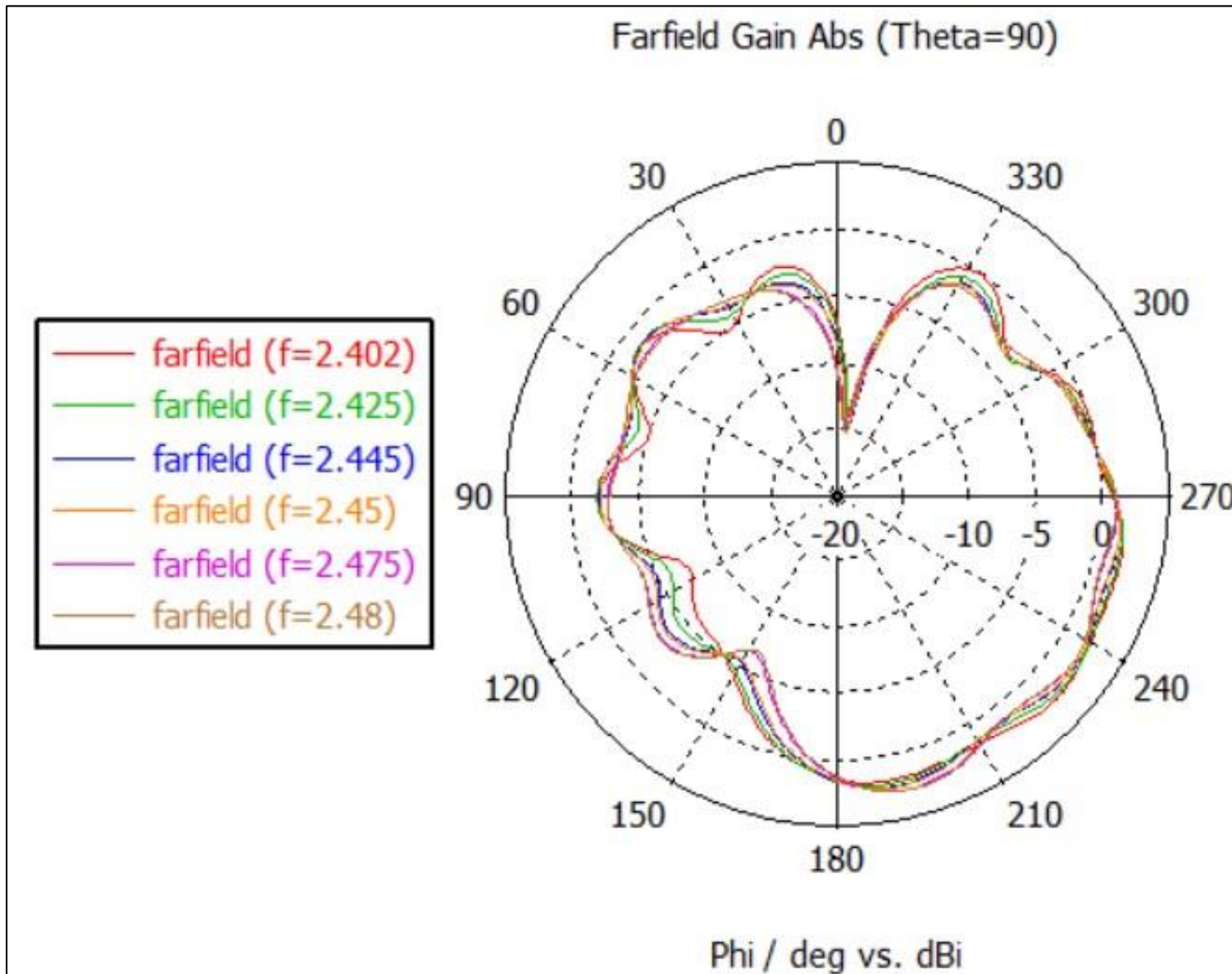
Figure 5: Excitation [1] _Theta=90_farfield cuts (f=2.402, 2.45, and 2.480 GHz)
