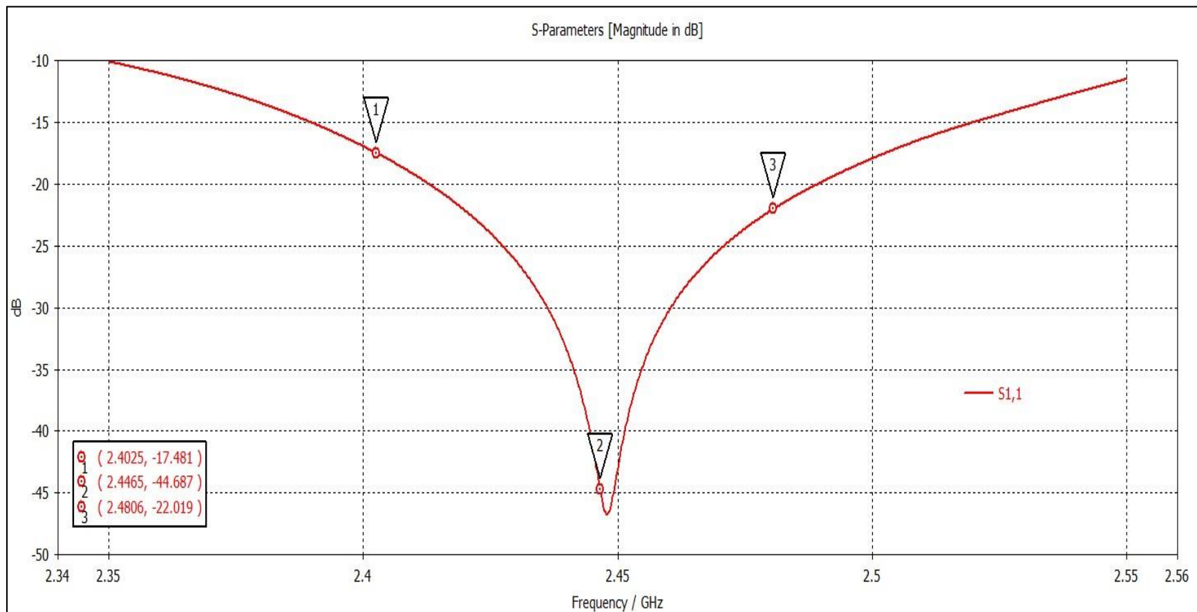
Figure 2: BT/BLE Antenna 1D Results - S-Parameters- S1 1
