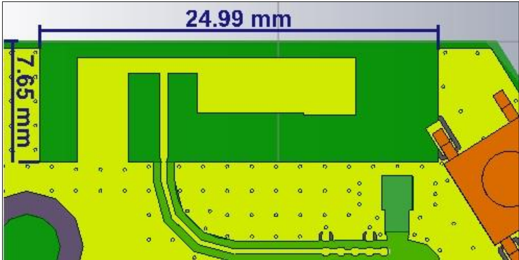
Figure 1: WMJ4 BT Antenna dimensions
