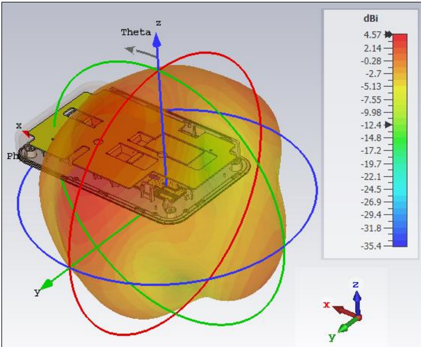
Figure 4: Farfield radiation pattern at 2.445 GHz
