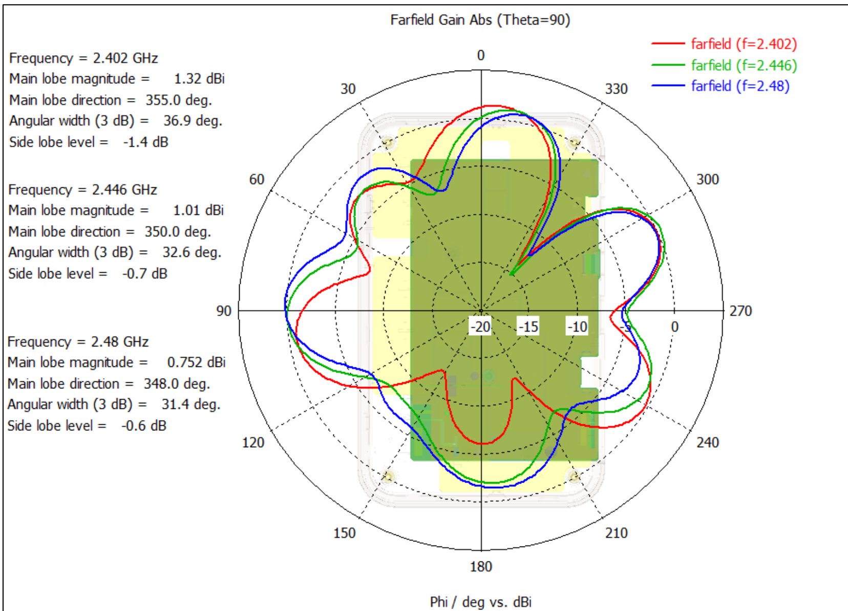
Figure 5: Excitation [1] _Theta=90_farfield cuts (f=2.402, 2.45, and 2.480 GHz)
