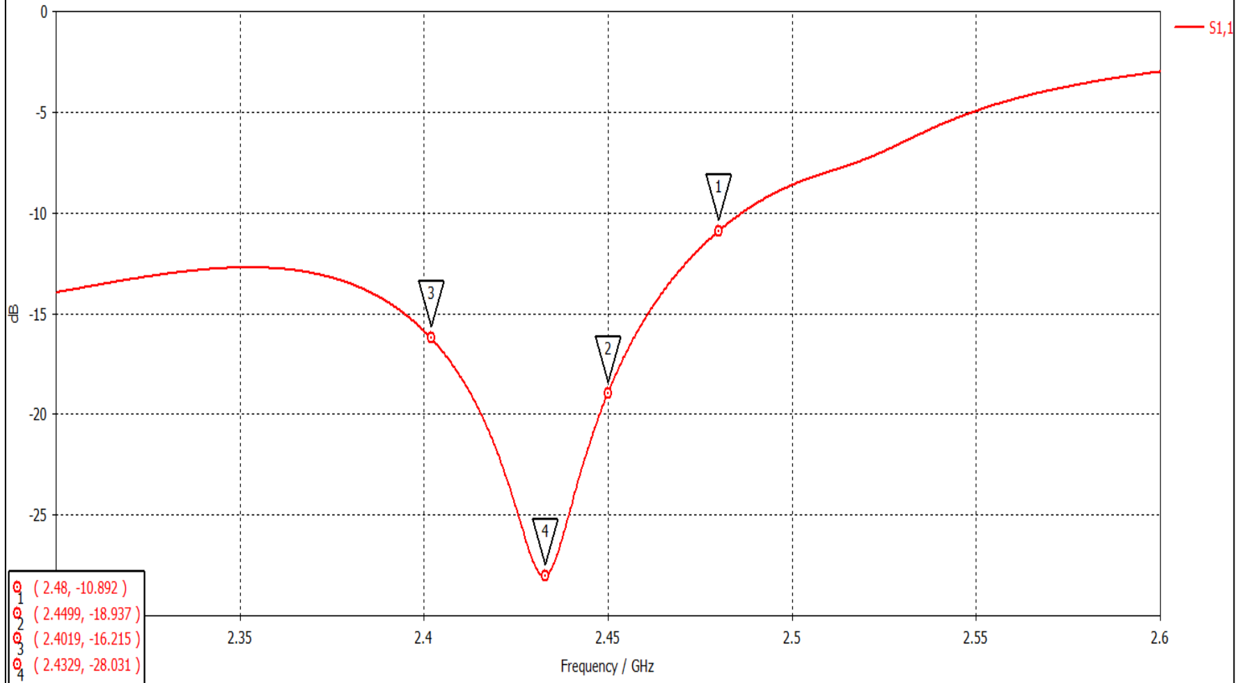
S-Parameters [Magnitude in dB]
