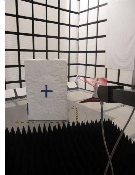
RADIATED FRONT PHOTO (ABOVE 1 GHz)
