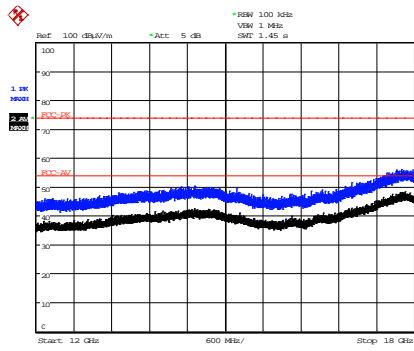
Date: 6.JUL.2016 15:10:06 12 GHz – 18 GHz
