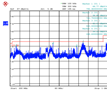
Date: 4.JUL.2016 17:49:14 200 MHz – 1 GHz
