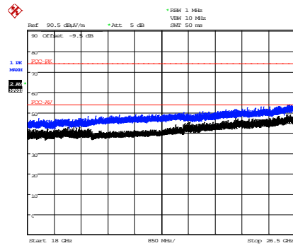
Date: 6.JUL.2016 16:19:30 18 GHz – 26.5 GHz
