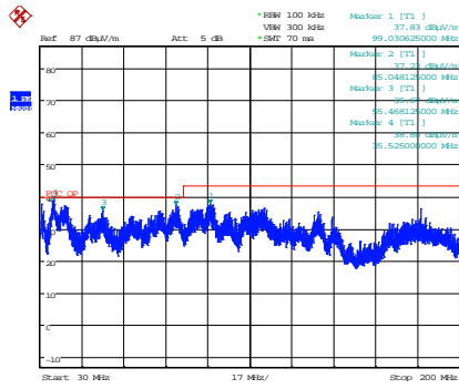
Date: 4.JUL.2016 10:16:42 30 MHz – 200 MHz
