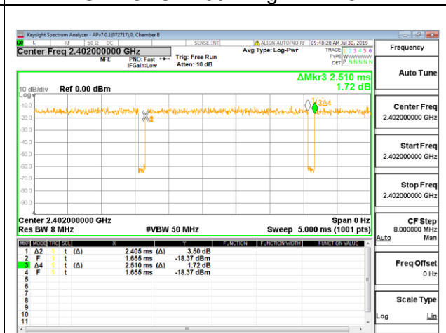
DUTY CYCLE 802.11n HT20 2TX MODE
