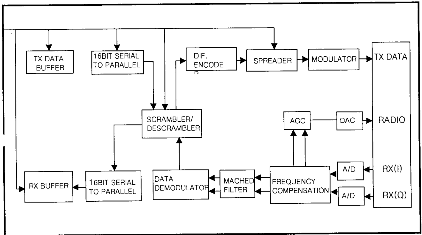
DCT Spread Spectrum Engine Block Diagram
