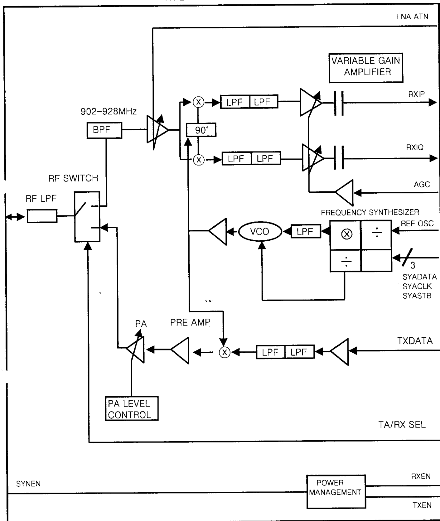
MH-9988 RF BLOCK DIAGRAM
