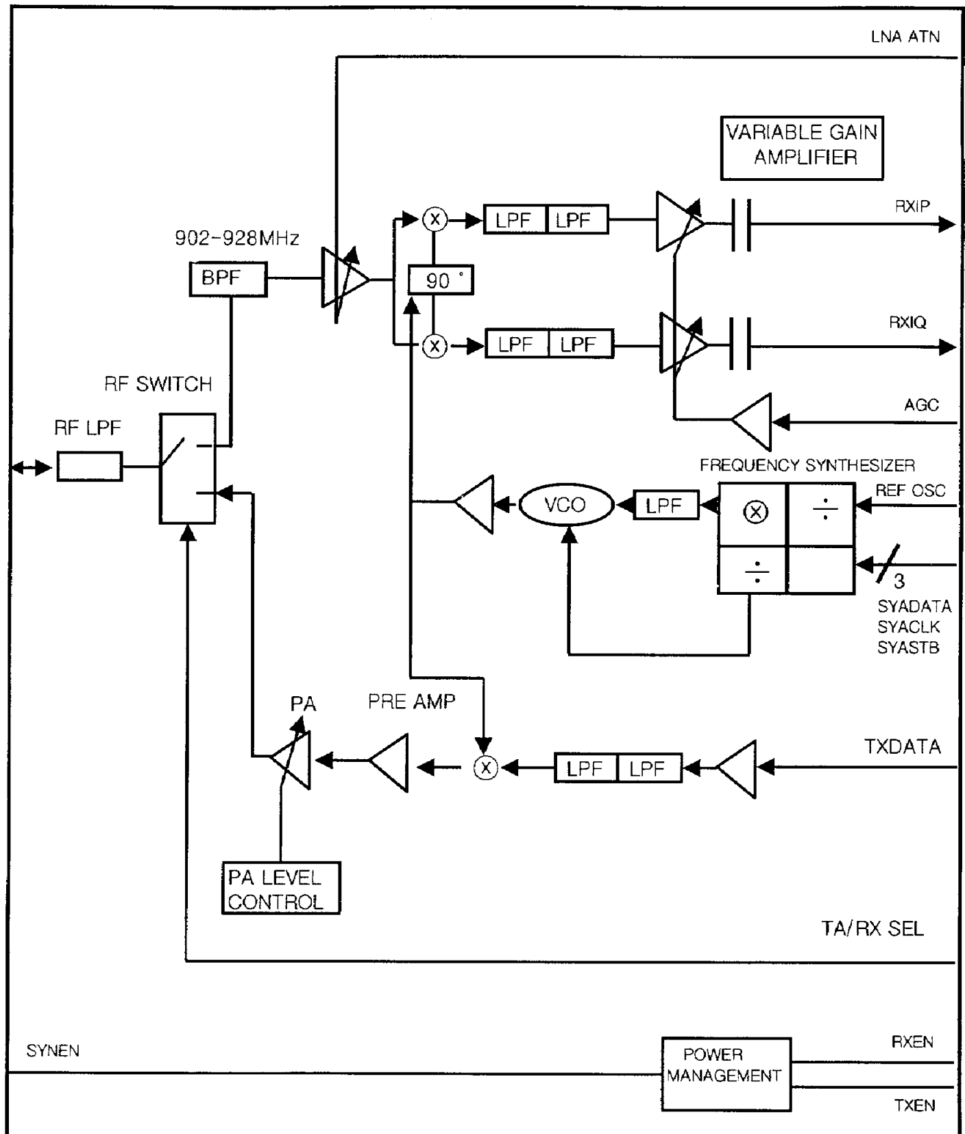
MH-9082 RF BLOCK DIAGRAM
